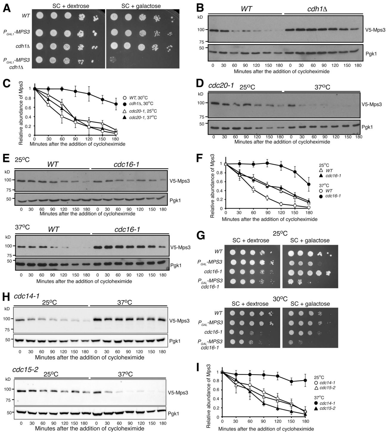
Figure 5. APC/C Cdh1 -dependent regulation of Mps3 degradation. (A) MPS3 genetically interacts with CDH1 . To determine cell viability, yeast cells were grown overnight in YPD liquid medium to reach saturation, 10-fold diluted, spotted onto SC plates with either 2% dextrose or 2% galactose, and then incubated at 30°C for ~2 d. Overexpression of MPS3 is lethal in cdh1Δ cells. (B) The APC/C activator, Cdh1, regulates Mps3 degradation. The relative protein abundance of Mps3 in WT and cdh1Δ cells was analyzed after arresting cells in G1 using \alpha factor (10 \mu g/ml) for 2 h, and then CHX chase was performed as described in Fig. 1A. (C) Quantification of the relative abundance of Mps3 as shown in B and D. Representative blots from three biological replicates of each experiment are shown. (D) Mps3 turnover is independent of Cdc20. Cells were grown at 25°C to the exponential phase, and CHX was then added as shown in Fig. 1A. To inactivate cdc20-1 , cells were shifted to 37°C for 1 h before the addition of CHX. (E and F) The APC/C subunit Cdc16 regulates Mps3 degradation. Cells were grown at 25°C to the exponential phase, and CHX was then added as shown in Fig. 1A. To inactivate cdc16-1 , cells were shifted to 37°C for 1 h before the addition of CHX. Quantification of Mps3 protein abundance is shown in F. Error bars represent the standard deviation from the mean of biological replicates ( n = 3 ). Notably, inactivation of the APC through the cdc16-1 allele at the nonpermissive temperature resulted in a threefold increase in Mps3 half-life. (G and H) MPS3 genetically interacts with cdc16-1 . Overexpression of MPS3 in cdc16-1 cells showed a sick phenotype at a semipermissive temperature. Yeast cells were grown overnight in YPD liquid medium to reach saturation, 10-fold diluted, spotted onto SC plates with either 2% dextrose or 2% galactose, and then incubated at
