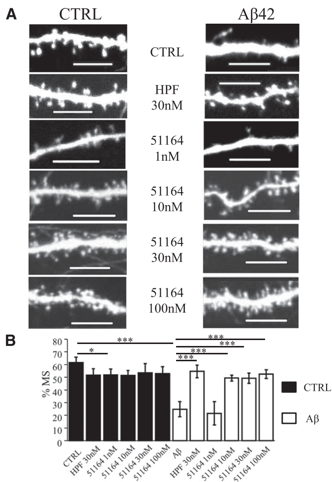
Fig. 4. Evaluation of the protective effects of compound 51164 in conditions of amyloid synaptotoxicity. (A) Representative confocal images of day 14 of in vitro cultivation hippocampal neurons transfected with tdTomato plasmid. Images for control (CTRL) cultures and cultures exposed to oligomeric Aβ42 (Aβ) are shown as indicated. HPF was added at the concentration of 30 nM, compound 51164 was tested at concentrations of 1, 10, 30, and 100 nM as indicated. Scale bar, 10 μm. (B) The average percentages of mushroom spines (%MS) in each experimental condition are present as mean ± S.D. ( n = 22 – 32 neurons for each group). Untreated hippocampal cultures (CTRL) are shown as filled bars. Open bars correspond to hippocampal cultures that were treated with oligomeric Aβ42. ^{*}P < 0.05 ; ^{***}P < 0.0005 by two-way ANOVA with Dunn-Sidak post hoc test.
