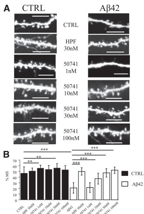
Fig. 3. Evaluation of protective effects of compound 50741 in conditions of amyloid synaptotoxicity. (A) Representative confocal images of day 14 of in vitro cultivation hippocampal neurons transfected with tdTomato plasmid. Images for control (CTRL) cultures and cultures exposed to oligomeric Aβ42 are shown as indicated. HPF was added at the concentration of 30 nM, compound 50741 was tested at concentrations of 1, 10, 30, and 100 nM as indicated. Scale bar, 10 μm. (B) The average percentages of mushroom spines (%MS) in each experimental condition are present as mean ± S.D. ( n = 22 – 32 neurons for each group). Untreated hippocampal cultures (CTRL) are shown as filled bars. Open bars correspond to hippocampal cultures that were treated with oligomeric Aβ42. ^{*}P < 0.005 ; ^{***}P < 0.0005 by two-way ANOVA with Dunn-Sidak post hoc test.
