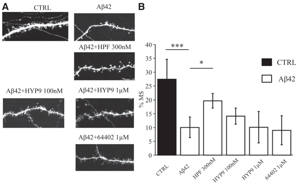
Fig. 2. Evaluation of protective effects of HYP9 and compound 64402 in conditions of amyloid synaptotoxicity. (A) Representative confocal images of day 14 of in vitro cultivated hippocampal neurons transfected with tdTomato plasmid. Images for control (CTRL) cultures and cultures exposed to oligomeric A \beta 42 are shown as indicated. HPF was added at the concentration of 300 nM, HYP9 was tested at concentrations of 100 nM and 1 \mu M as indicated, compound 64402 was tested at the 1 \mu M concentration. (B) The average percentages of mushroom spines (%MS) in each experimental condition are present as mean \pm S.D. ( n \geq 16 neurons for each group). Untreated hippocampal cultures (CTRL) are shown as the filled bar. Open bars correspond to hippocampal cultures that were treated with oligomeric A \beta 42. * P < 0.05 ; *** P < 0.0005 by one-way ANOVA, following Dunn-Sidak post hoc test.
