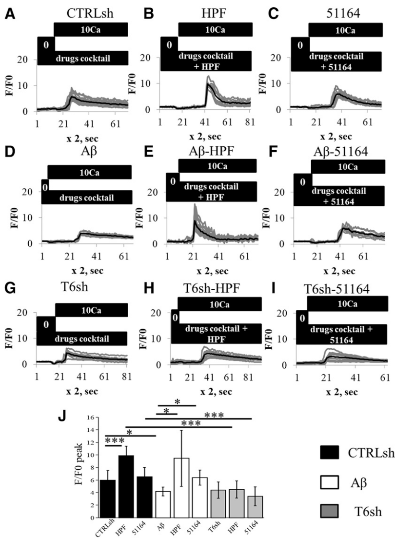
Fig. 6. Compound 51164 rescues A\beta_{42} -suppressed nSOCE in hippocampal postsynaptic dendritic spines. (A–I) The time course of GCaMP5.3 fluorescence signal changes in the spines of hippocampal neurons at day 14 of in vitro cultivation. Neurons were preincubated in Ca^{2+} free media, and 10 mM Ca^{2+} was added as indicated by the black bar above the traces. The experiments were performed in the presence of a drug cocktail of Ca^{2+} inhibitors as described in Materials and Methods . The presence of 300 nM HPF or 300 nM of compound 51164 is indicated above the GCaMP5.3 traces. For each experimental group, individual spine (thin gray lines) and average (thick black lines) fluorescence traces are shown. Results with control (CTRL) neurons are shown in (A–C). Results with neurons preincubated with A\beta_{42} oligomers ( A\beta ) are shown in (D–F) as indicated. Results depicted in (A–F) were obtained in the presence of control shRNA (CTRLsh). Results with neurons transfected with shTRPC6 (T6sh) plasmids are shown in (G–I). (J) The average nSOCE spine peak amplitude is shown for each group of cells depicted in (A–I). The F/F_0 changes in GCaMP5.3 fluorescence are presented as mean \pm S.D. ( n = 20 spines), * P < 0.05 ; *** P < 0.0005 by Kruskal-Wallis ANOVA.
