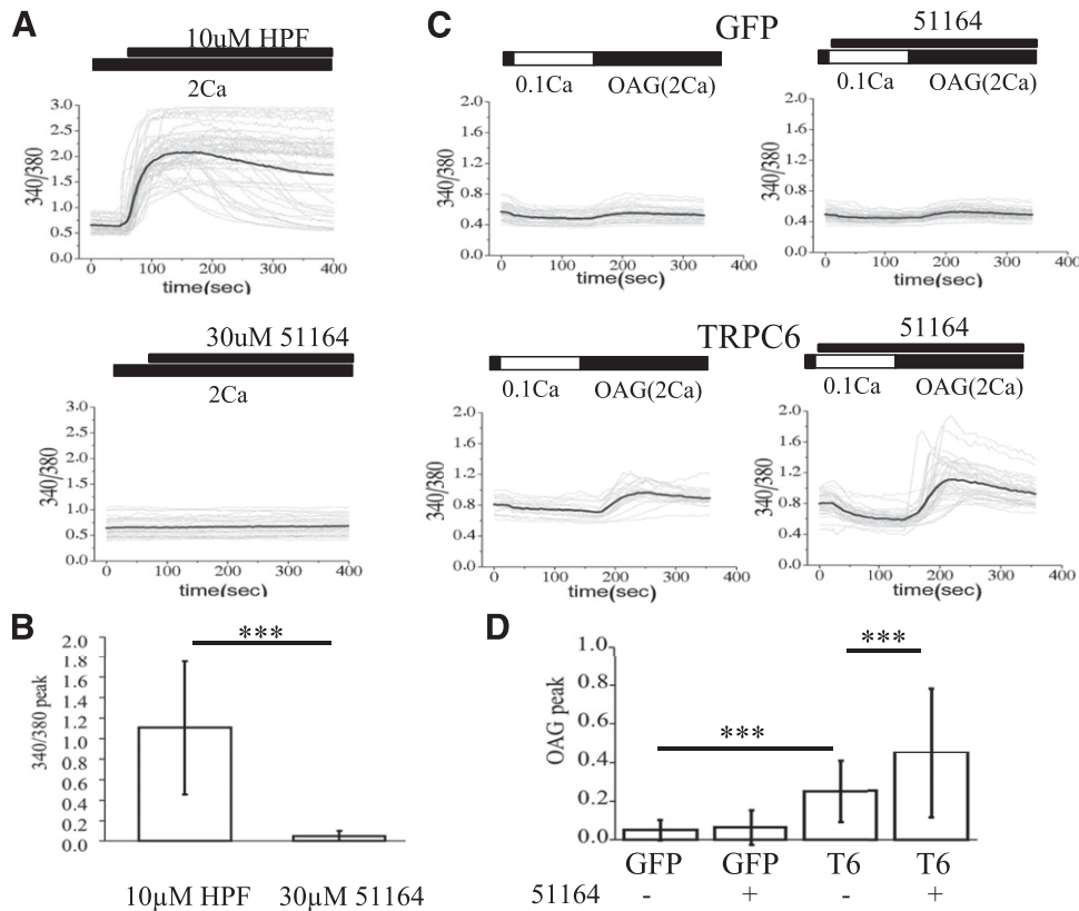
Fig. 5. Compound 51164 acts as a positive modulator of TRPC6 channels. (A) Time course of Fura-2 fluorescence Ca^{2+} signals (340/380 ratio) is shown for HEK293 cells transfected with EGFP + TRPC6 plasmids. Traces from individual cells are shown as thin gray lines, and average traces are shown as thick black lines. Cells were incubated in aCSF medium containing 2 mM Ca^{2+} . The time of addition of 10 \mu M HPF or 30 \mu M of compound 51164 is indicated by black bars above the Fura-2 traces. (B) Average amplitude of Ca^{2+} influx peak is shown as the change in 340/380 Fura-2 ratio signals for the cells exposed to HPF or compound 51164. The results are presented as mean \pm S.D. ( n = 40 cells). *** P < 0.0001 by two-way ANOVA with Tukey's post hoc test. (C) Time course of Fura-2 fluorescence Ca^{2+} signals (340/380 ratio) is shown for HEK293 cells transfected with EGFP (GFP) or EGFP + TRPC6 (TRPC6) plasmids as indicated. Traces from individual cells are shown as thin gray lines, and average traces are shown as thick black lines. Cells were moved to modified aCSF medium containing 0.1 mM Ca^{2+} for 2 minutes, and then returned to the medium containing 2 mM Ca^{2+} with the addition of 50 \mu M of OAG. The time of addition of 30 \mu M of compound 51164 is indicated by black bars above the Fura-2 traces. (D) Average amplitude of Ca^{2+} influx peak is shown as the change in 340/380 Fura-2 ratio signals for each group of cells tested in experiments shown in (C). The results are presented as mean \pm S.D. ( n = 40 cells). *** P < 0.0001 by two-way ANOVA with Tukey's post hoc test.
