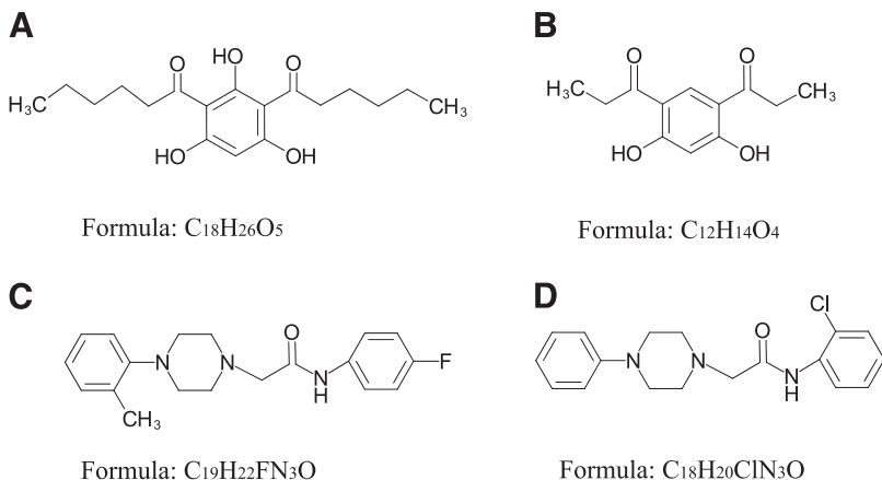
Fig. 1. Chemical structures of potential TRPC6 modulators identified as a result of bioinformatics search. (A) HYP-9, (B) compound 64402, (C) compound 50741, and (D) compound 51164. Compounds 64402, 50741, and 51164 were found in the InterBioScreen library.
