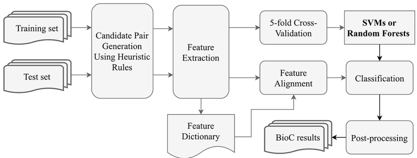
Figure 2. The workflow of relation extraction module.
