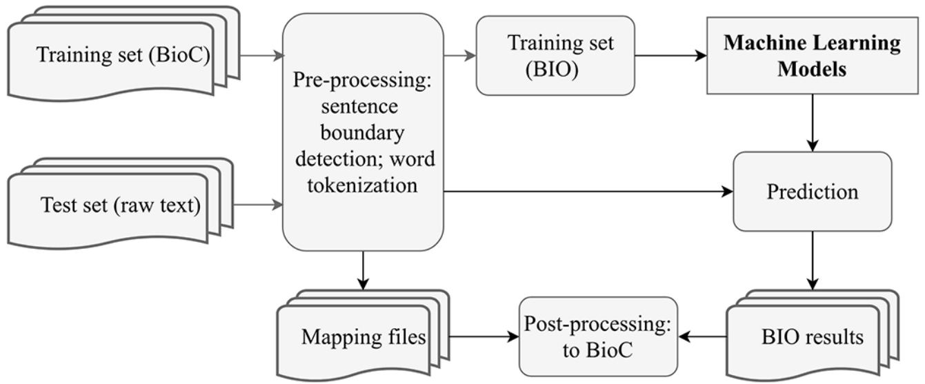
Figure 1. The workflow of NER module.
