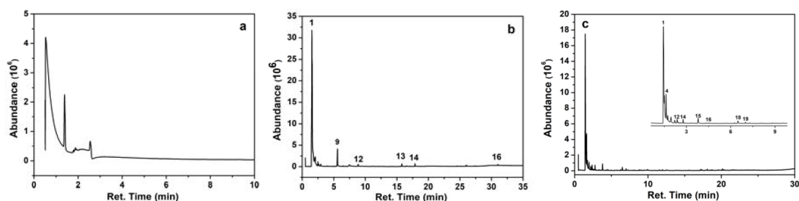
Figure 6. Py-GC-MS spectra of CAB at 200 °C (a), 400 °C (b), and 750 °C (c). The inset in (c) is the magnified spectrum of retention time within 9.5 min.
