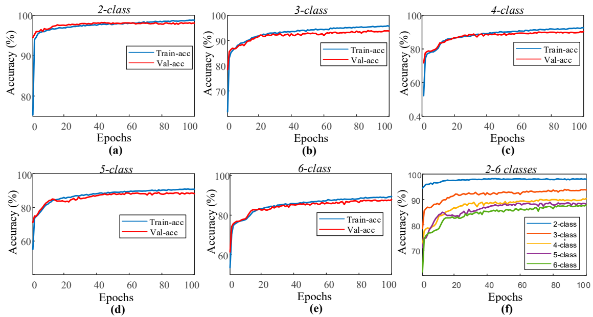
Figure 4. Performance graphs of the proposed 1D-CNN model with the single EOG signal for the sleep-edf dataset: (a) two-class model, (b) three-class model, (c) four-class model, (d) five-class model, (e) six-class model, and (f) validation accuracy for the models with two to six classes.
