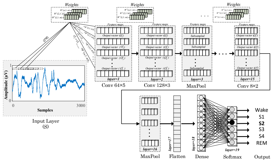
Figure 2. Block representation of the proposed one-dimensional convolutional neural network (1D-CNN) model for the classification of sleep stages.
