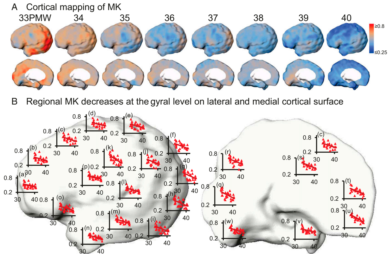
Fig. 1. (A) Spatiotemporal maps of cortical MK measurements of preterm brains at eight consecutive time points from 33 to 40 PMW displayed on a partially inflated cortical surface of a template brain. (B) Linear fitting of MK time courses at different cortical gyri overlaid onto the template brain in the left hemisphere displayed in lateral (Left) and medial (Right) view. In each scatter plot, the x axis indicates postmenstrual age in PMW, and the y axis indicates MK values. The cortical gyri underlying the scatter plots are listed below: a, inferior frontal; b, middle frontal; c, superior frontal; d, precentral; e, postcentral; f, superior parietal; g, superior occipital; h, middle occipital; i, inferior occipital; k, angular; j, supramarginal; l, superior temporal; m, middle temporal; n, inferior temporal; o, lateral orbitofrontal; p, insula; q, cuneus; r, precuneus; s, cingulate; t, medial orbitofrontal; u, gyrus rectus; v, fusiform; w, lingual.
