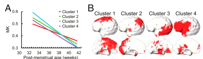
Fig. 3. (A) The MK time courses of four clusters identified by NMF. (B) The respective locations of the four clusters on the cortical surface.
