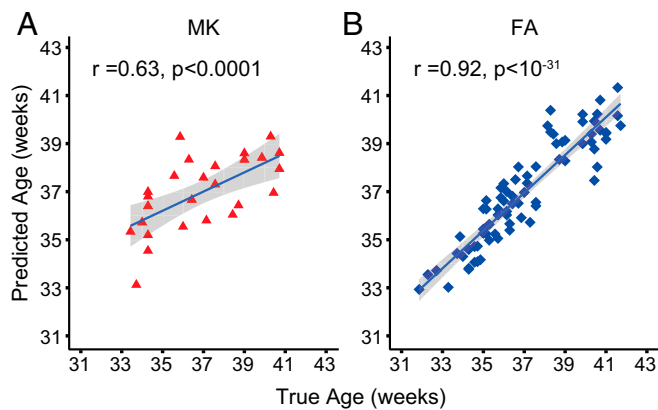
Fig. 6. Age prediction of the preterm neonates with cortical MK (A) and FA (B) measurements.
