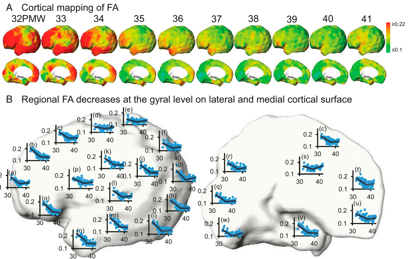
Fig. 2. (A) Spatiotemporal maps of cortical FA measurements of preterm brains at 10 consecutive time points from 32 to 41 PMW displayed on a partially inflated cortical surface of a template brain. (B) Biphasic linear fitting of FA time courses at different cortical gyrus overlaid onto the template brain in the left hemisphere displayed in lateral ( Left ) and medial ( Right ) view. In each scatter plot, the x axis indicates postmenstrual age in PMW, and the y axis indicates FA values. The cortical gyri underlying the scatter plots are the same as those shown in Fig. 1B.
