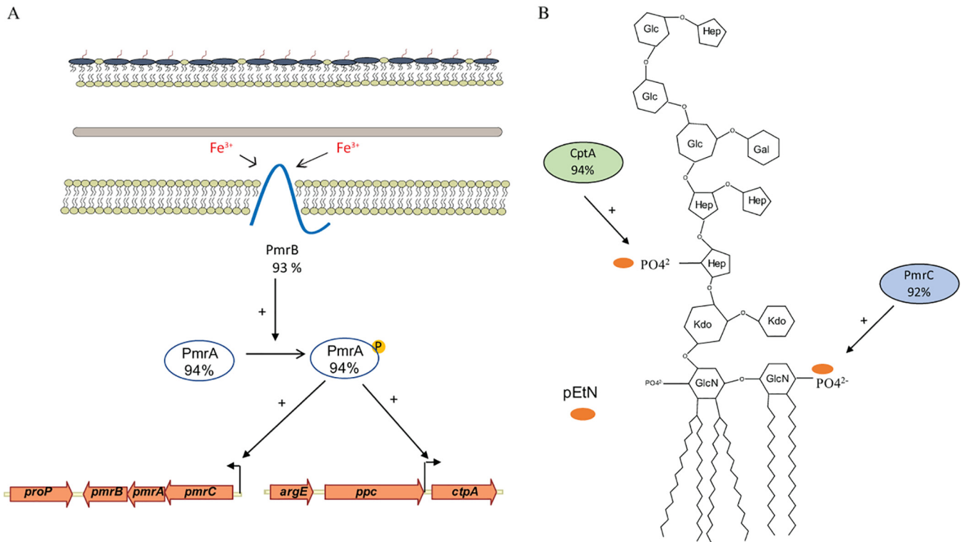
FIG 1 PmrAB regulates pmrC ( eptA ) and cptA in C. rodentium . (A) Model representing the PmrAB TCS. Under conditions of high \text{Fe}^{3+} , the cytoplasmic PmrA response regulator becomes phosphorylated and active, resulting in differential expression of several genes, including pmrC ( eptA ) and cptA (31). (B) Schema showing PmrC (EptA) and CptA-mediated modifications of LPS. In E. coli , PmrC (EptA) and CptA add pEtN groups to the lipid A and core regions of LPS, respectively (36). Percentages refer to the similarity of the PmrA, PmrC (EptA), and CptA proteins between E. coli and C. rodentium .
