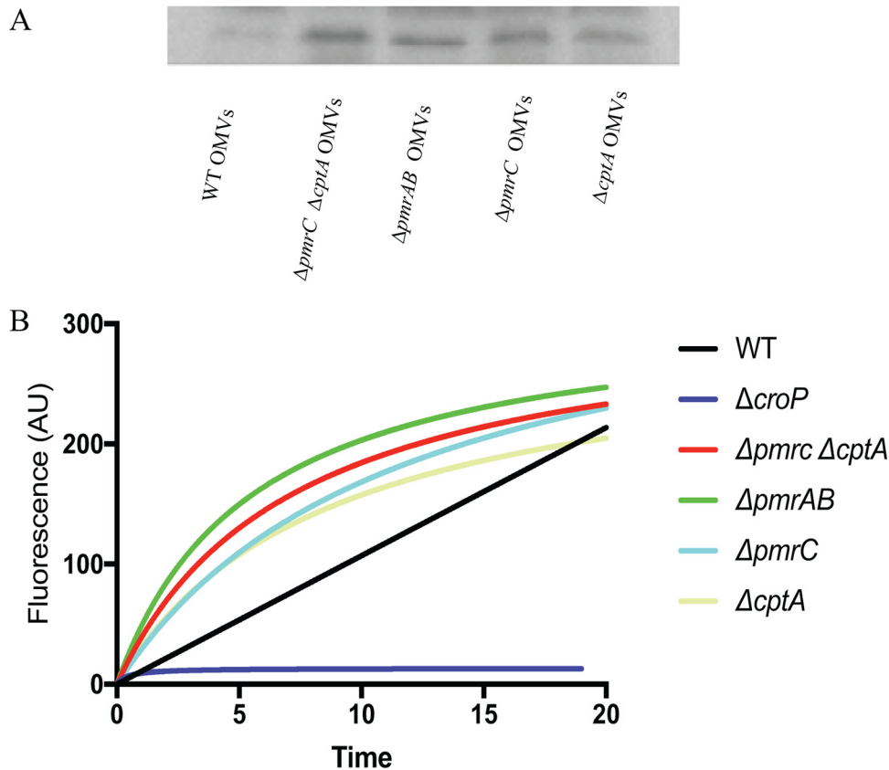
FIG 8 The outer membrane protease CroP is present in C. rodentium OMVs. OMVs were isolated from C. rodentium strains grown to mid-log phase in the presence of 50 \mu\text{M} \text{FeCl}_2 . (A) The relative amounts of CroP found within equal volumes of isolated OMVs were determined by Western blotting using an anti-CroP antibody. (B) CroP activity of OMVs were assessed by incubating equal volumes of OMVs isolated from different C. rodentium strains with the C2 FRET substrate for 20 min. Cleavage of the FRET substrate was determined by measuring relative fluorescence at 430 nm after excitation at 325 nm. Data shown are representative of three independent experiments. Data were fitted to a Michaelis-Menten nonlinear regression curve using GraphPad Prism 7 software.
