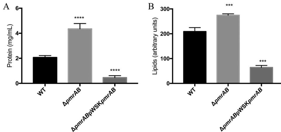
FIG 2 Deletion of the pmrAB TCS genes results in increased OMV biogenesis in C. rodentium . OMVs isolated from the C. rodentium wild-type, \Delta pmrAB , and \Delta pmrAB pWSK pmrAB strains grown in the presence of 50 \mu M FeCl_2 were quantified by measuring protein and lipid contents (A) Protein content of OMVs was measured using the DC protein assay. Protein concentration was calculated using BSA as a standard. (B) The lipid content of OMV samples was determined by using the lipophilic dye FM 1-43. Cultures were grown to mid-log phase and normalized to an OD_{595} of 0.5 prior to OMV isolation. Values shown are the means \pm standard error from three independent experiments. Significance was assessed relative to wild-type using one-way ANOVA; ****, P \leq 0.0001 ; ***, P \leq 0.001 .
