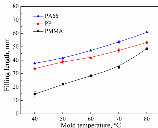
Figure 6. Effect of mold temperature on the filling length of polymer melt (UA = 40 μm, PPe = 14 MPa, UT = 6 s, HT = 6 s, HP = 14 MPa; Mold I).
