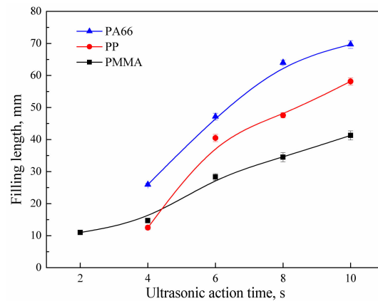
Figure 3. Influence of ultrasonic action time on the filling length of polymer melt (UA = 40 \mu\text{m} , PPe = 14 MPa, HT = 6 s, HP = 14 MPa, MT = 60 ^{\circ}\text{C} ; Mold I).
