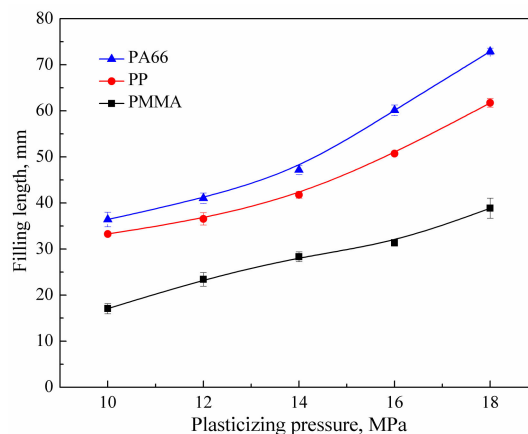
Figure 4. Effects of plasticizing pressure on the filling length of polymer melt (UA = 40 \mu\text{m} , UT = 6 s, HT = 6 s, HP = 14 MPa, MT = 60 ^{\circ}\text{C} ; Mold I).
