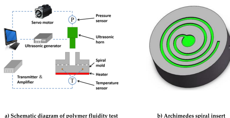
Figure 1. Ultrasonic microinjection molding equipment.
