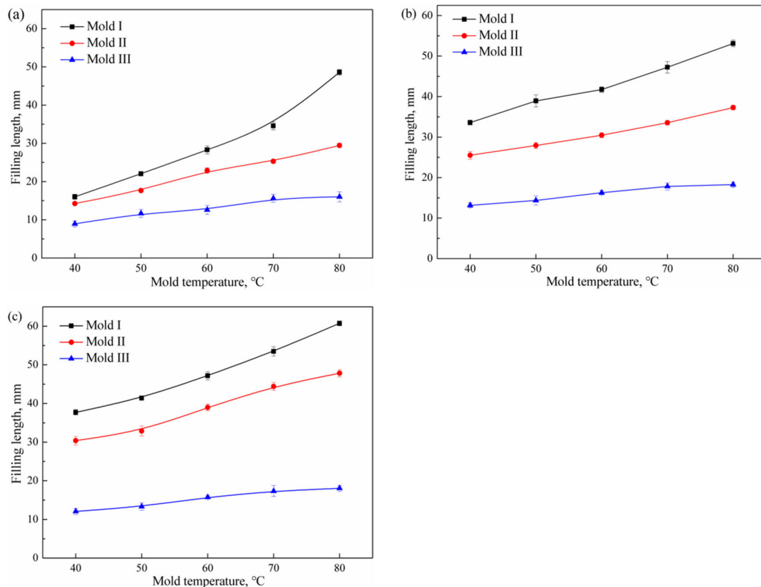
Figure 7. Filling length of polymer melt in different mold (a) PMMA; (b) PP; (c) PA66.
