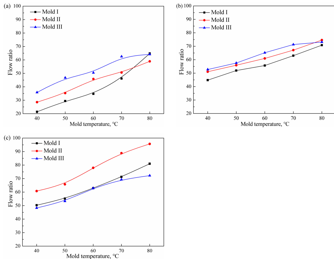
Figure 8. Flow ratios of polymers in different molds (a) PMMA; (b) PP; (c) PA66.
