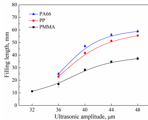
Figure 2. Influence of ultrasonic amplitude on the filling length of polymer melt (UT = 6 s, PPe = 14 MPa, HT = 6 s, HP = 14 MPa, MT = 60 °C; Mold I).
