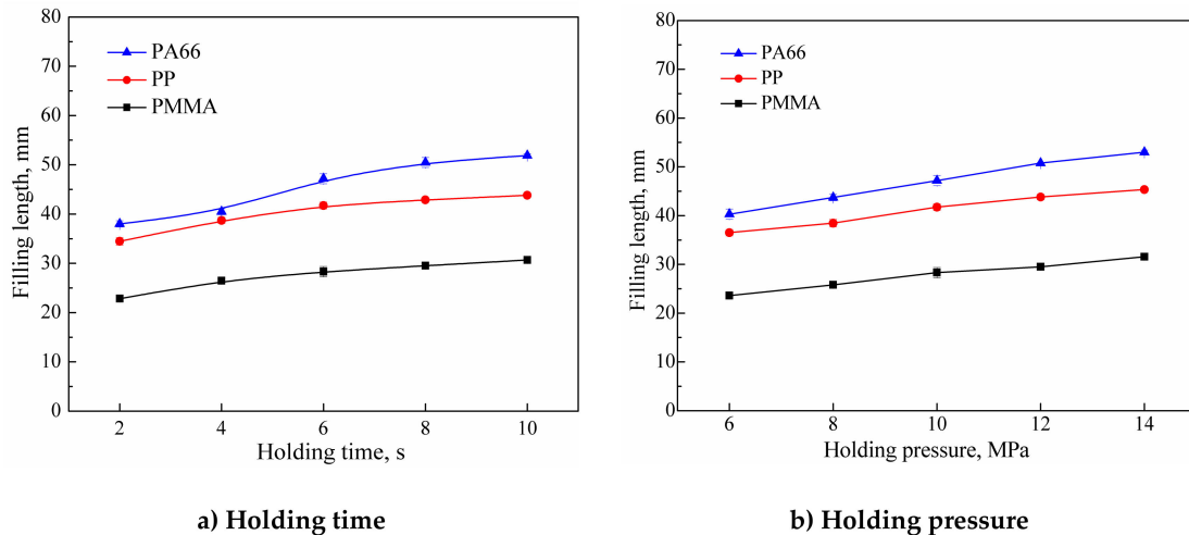
Figure 5. Effects of the holding process on the filling length of polymer melt (UA = 40 μm, UT = 6 s, PPe = 14 MPa, MT = 60 °C; Mold I).
