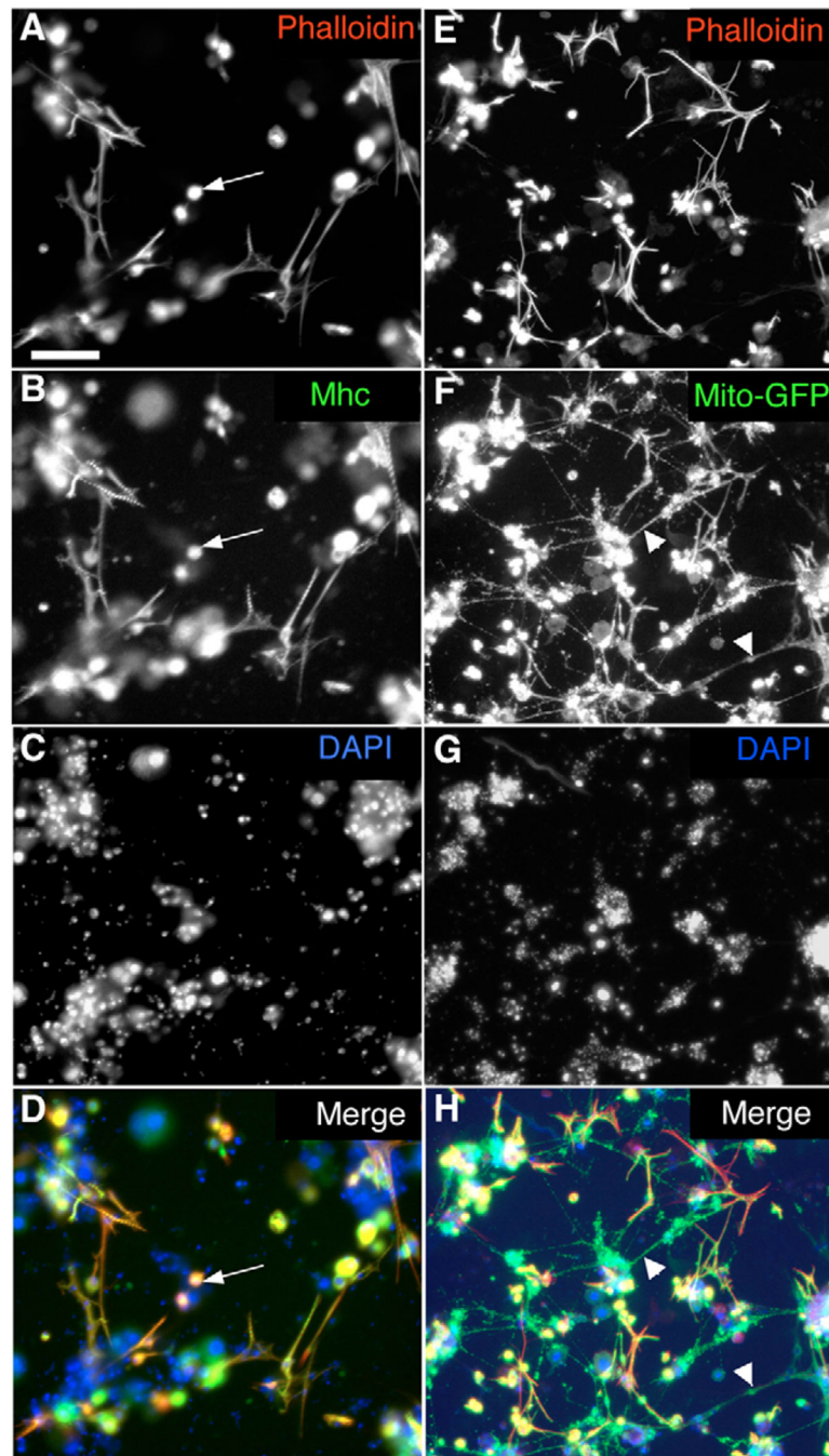
Fig. 2. Primary cultures derived from Drosophila embryonic cells contain a mixture of different cell populations that include muscles and neurons.
