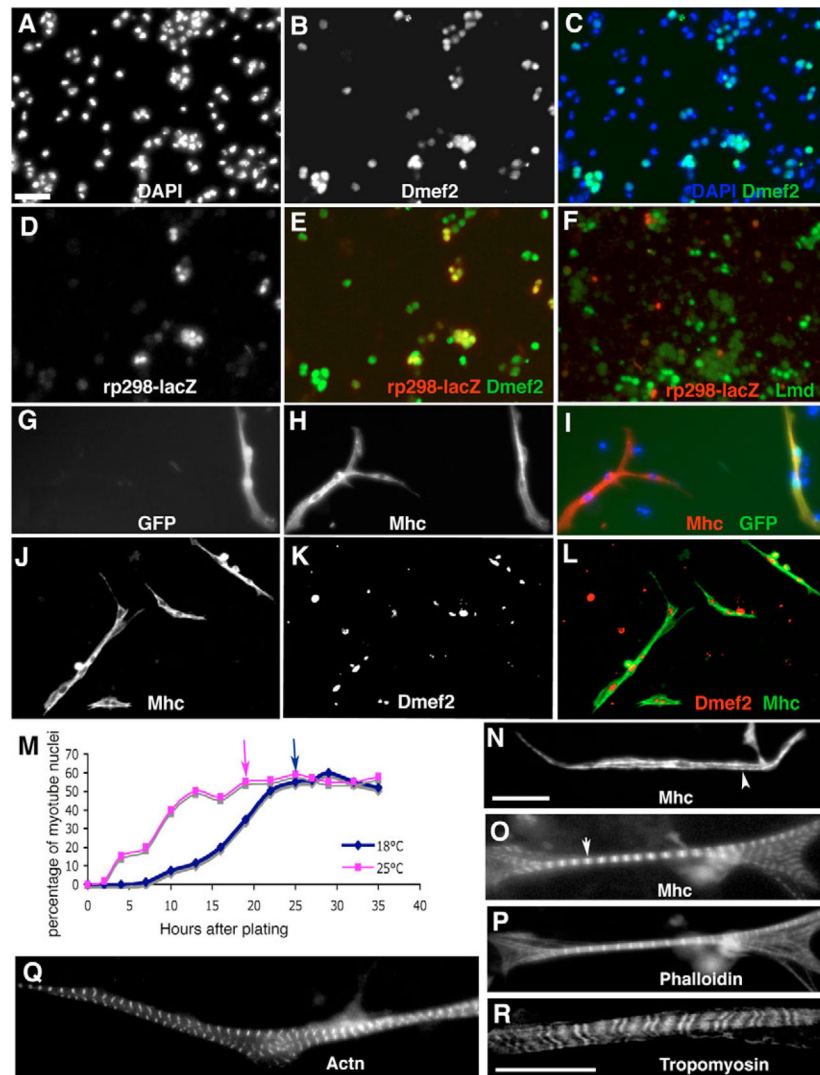
Fig. 1. Myogenesis in primary cultures derived from Drosophila embryos.
