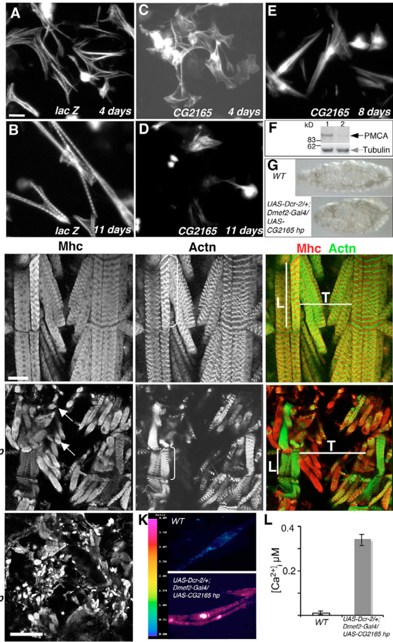
Fig. 6. In vivo validation of CG2165 using transgenic RNAi.
