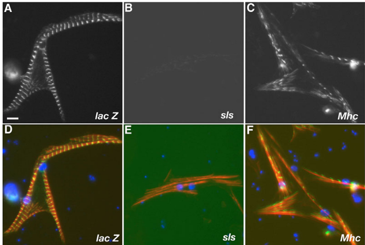
Fig. 3. Gene-specific RNAi effects in primary cells.
