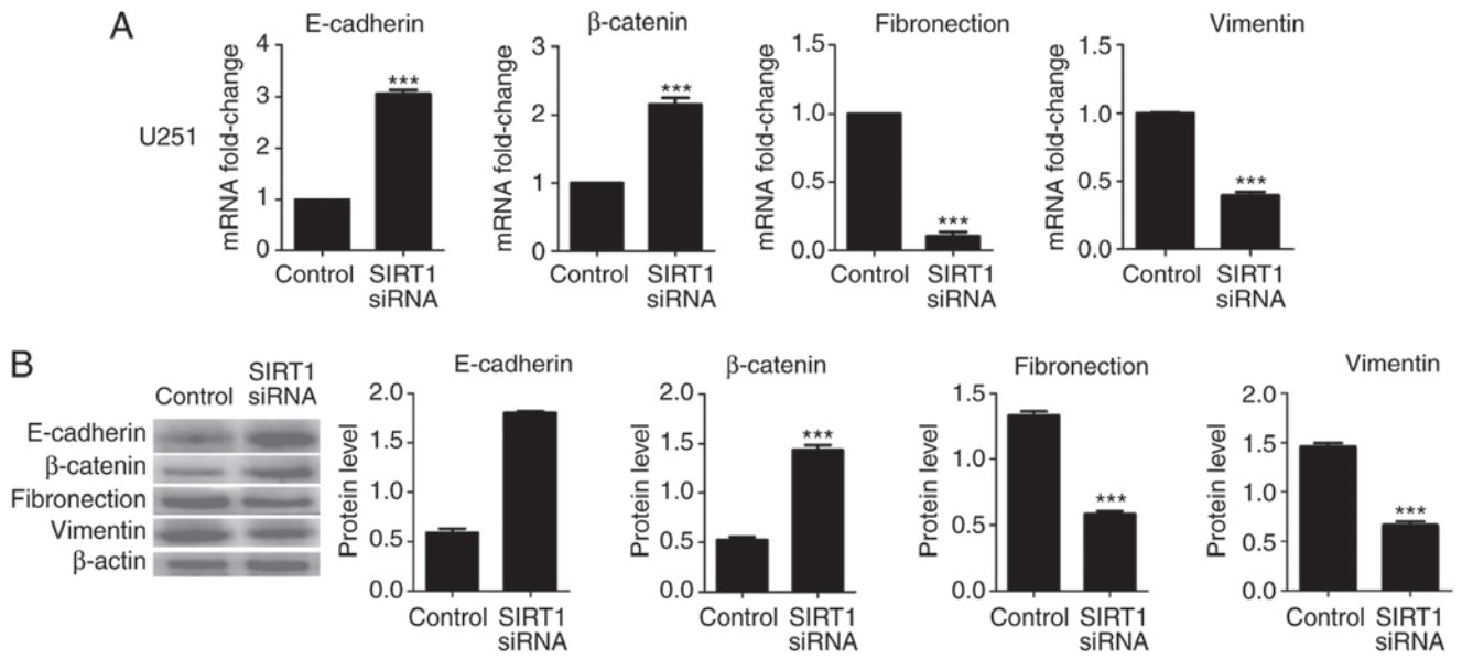
Figure 5. SIRT1 silencing inhibits epithelial-mesenchymal transition in U251 cells. The (A) mRNA and (B) protein levels of E-cadherin, \beta -catenin, fibronectin and vimentin in U251 cells following transfection with SIRT1-siRNA were determined using the reverse transcription-quantitative polymerase chain reaction and western blotting, respectively. *** P < 0.001 . siRNA, silencing RNA; SIRT1, silent information regulator 1; E-cadherin, epithelial cadherin.
