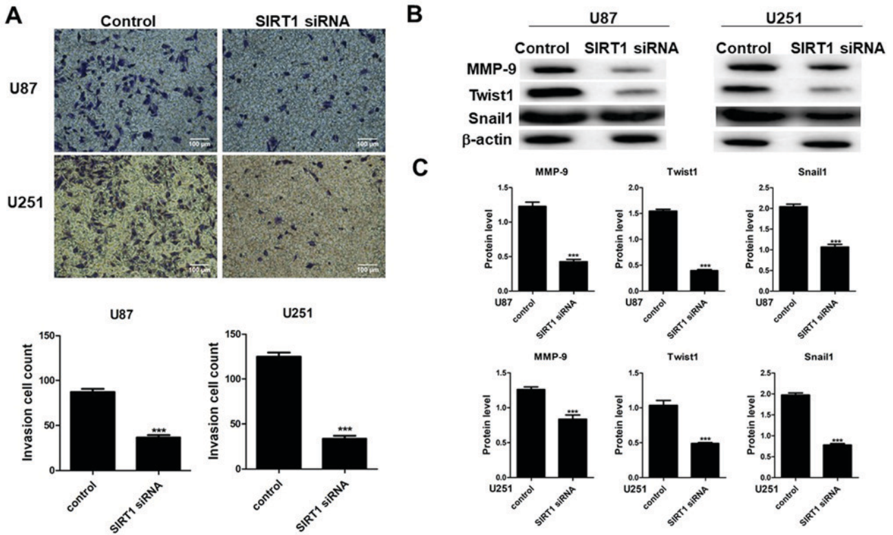
Figure 3. SIRT1 silencing inhibits invasion of glioma cells. (A) Invasive ability of U87 and U251 cells following transfection with SIRT1-siRNA determined using Transwell assays (magnification x100). (B) Western blotting of MMP-9, Twist1 and Snail1 in U87 and U251 cells following transfection with SIRT1-siRNA. (C) Quantification of protein levels. Results are presented as the mean \pm standard deviation of three independent experiments. ***P<0.001. MMP-9, matrix metalloproteinase-9; siRNA, small interfering RNA; SIRT1, silent information regulator 1, Snail1, snail family transcriptional repressor 1; Twist1, family basic helix-loop-helix transcription factor 1.
