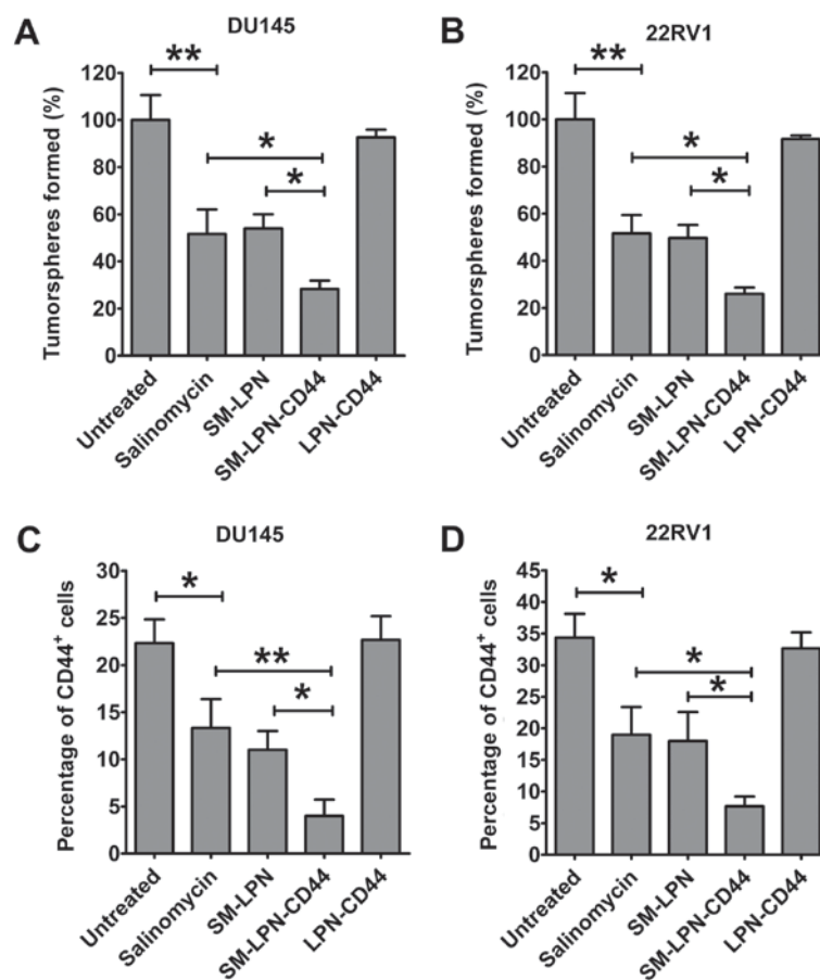
Figure 5. Impact of nanoparticles on the proportion of cancer-initiating cells in prostate cancer cells. Evaluation of tumorsphere formation in (A) DU145 and (B) 22RV1 cells following the treatment of prostate cancer cells and culture in serum-free medium. The percentage of CD44 + cells in (C) DU145 and (D) 22RV1 cells was evaluated by flow cytometry following treatment of prostate cancer cells. Data are presented as the mean \pm standard deviation (n=3). *P<0.05 and **P<0.01. SM-LPN-CD44, salinomycin-encapsulated lipid-poly(lactide-co-glycolide acid) nanoparticles linked with CD44 antibodies; SM-LPN, salinomycin-encapsulated lipid-poly(lactide-co-glycolide acid) nanoparticles; LPN-CD44, blank lipid-poly(lactide-co-glycolide acid) nanoparticles linked with CD44 antibodies.
