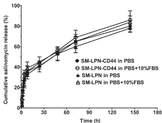
Figure 1. Salinomycin release from nanoparticles. The release media were PBS and PBS with 10% FBS. The accumulated salinomycin release rate of the nanoparticles was measured using the following formula: (M_t/M_i) \times 100 , where M_t is the mass of accumulated released salinomycin and M_i is the total amount of salinomycin. Data are presented as the mean \pm standard deviation (n=3). SM-LPN-CD44, salinomycin-encapsulated lipid-poly(lactide-co-glycolide acid) nanoparticles linked with CD44 antibodies; SM-LPN, salinomycin-encapsulated lipid-poly(lactide-co-glycolide acid) nanoparticles; FBS, fetal bovine serum.
