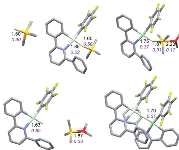
Fig. 5 Structure of the silane complex [\text{LAu}(\text{HSiMe}_3)]^+ and activation of HSiMe 3 by \text{LAu}^+/\text{OMe}_2 . Bond lengths in Å, Wiberg bond indexes shown in purple and italics.
