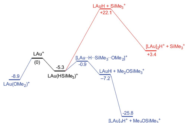
Fig. 4 Free energy profile of the reaction on \text{LAu}^+ with HSiMe 3 in the presence (black and blue parts) and absence (black and red parts) of OMe 2 .
