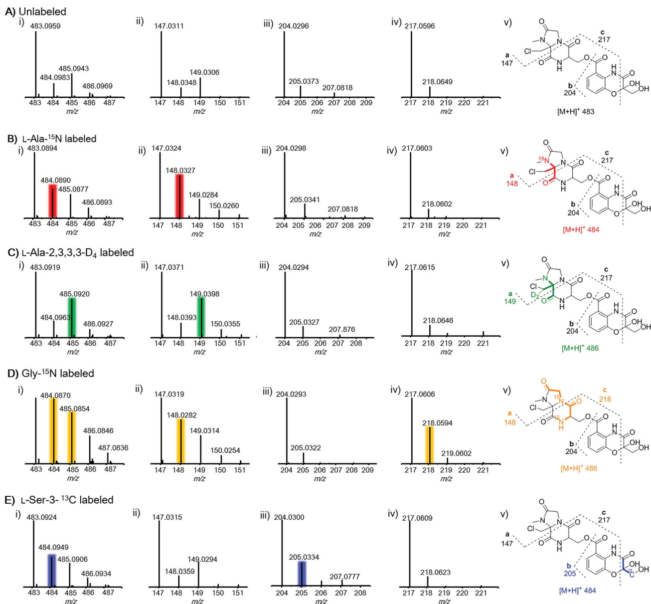
Fig. 3 MS and MS 2 fragmentation analysis of 2 when targeting the unlabeled (panel A) and after feeding with labeled amino acids including L -alanine- ^{15}\text{N} (panel B), L -alanine-2,3,3,3- \text{D}_4 (panel C), glycine- ^{15}\text{N} (panel D), and L -serine-3- ^{13}\text{C} (panel E). Panel (A): parent MS signal for unlabeled 2 (i, m/z 483, [\text{M} + \text{H}]^+ ); MS 2 ion signals for fragments of a (ii, m/z 147), b (iii, m/z 204), and c (iv, m/z 217); (v) MS 2 fragmentation ion pattern for unlabeled 2 . Panel (B): parent MS signal for 2 after feeding L -alanine- ^{15}\text{N} (i, m/z 484, [\text{M} + \text{H}]^+ ); MS 2 ion signals for fragments of a (ii, m/z 148), b (iii, m/z 204), and c (iv, m/z 217); (v) MS 2 fragmentation ion pattern for 2 after feeding L -alanine- ^{15}\text{N} . Panel (C): parent MS signal for 2 after feeding L -alanine-2,3,3,3- \text{D}_4 (i, m/z 484, [\text{M} + \text{H}]^+ ); MS 2 ion signals for fragments of a (ii, m/z 148), b (iii, m/z 204), and c (iv, m/z 217); (v) MS 2 fragmentation ion pattern for 2 after feeding L -alanine-2,3,3,3- \text{D}_4 . Panel (D): parent MS signal for 2 after feeding glycine- ^{15}\text{N} (i, m/z 485, [\text{M} + \text{H}]^+ ); MS 2 ion signals for fragments of a (ii, m/z 148), b (iii, m/z 204), and c (iv, m/z 218); (v) MS 2 fragmentation ion pattern for 2 after feeding glycine- ^{15}\text{N} . Panel (E): parent MS signal for 2 after feeding L -serine-3- ^{13}\text{C} (i, m/z 484, [\text{M} + \text{H}]^+ ); MS 2 ion signals for fragments of a (ii, m/z 147), b (iii, m/z 205), and c (iv, m/z 217); (v) MS 2 fragmentation ion pattern for 2 after feeding L -serine-3- ^{13}\text{C} .
