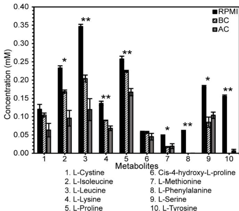
Figure 1. Initial Metabolite Concentration in Media Immediately after Treatment with Biochar or Activated Carbon.
