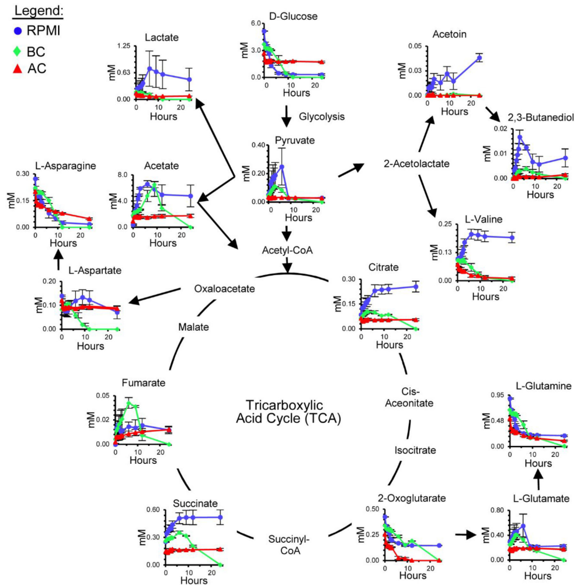
Figure 4. Tricarboxylic Acid (TCA) Cycle of E. coli .
