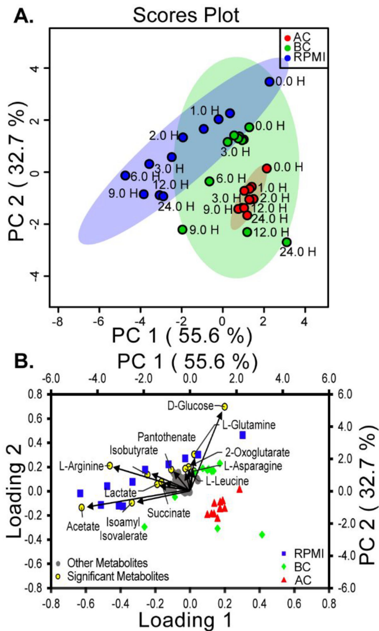
Figure 6. Statistical Analysis of E. coli in Unfiltered RPMI Media.
