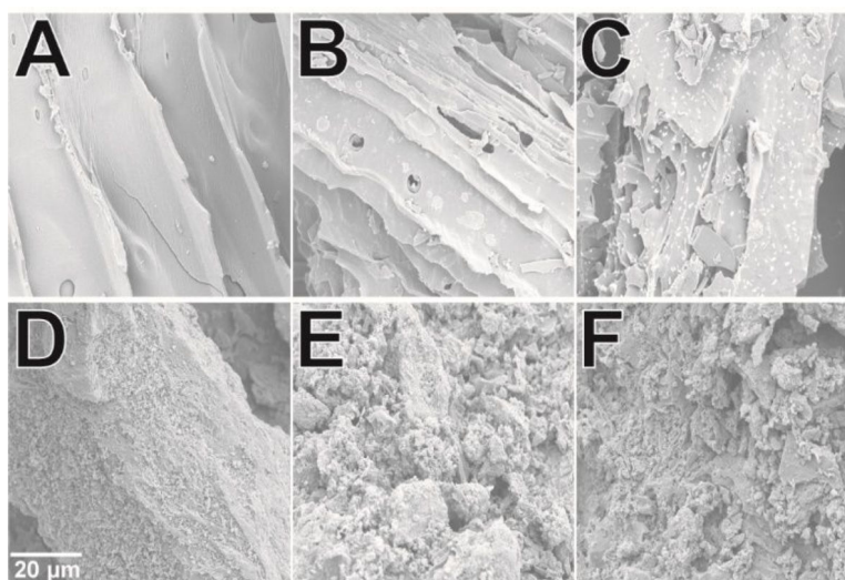
Figure 3. SEM of Bacterial Interactions with Biochar and Activated Carbon.
