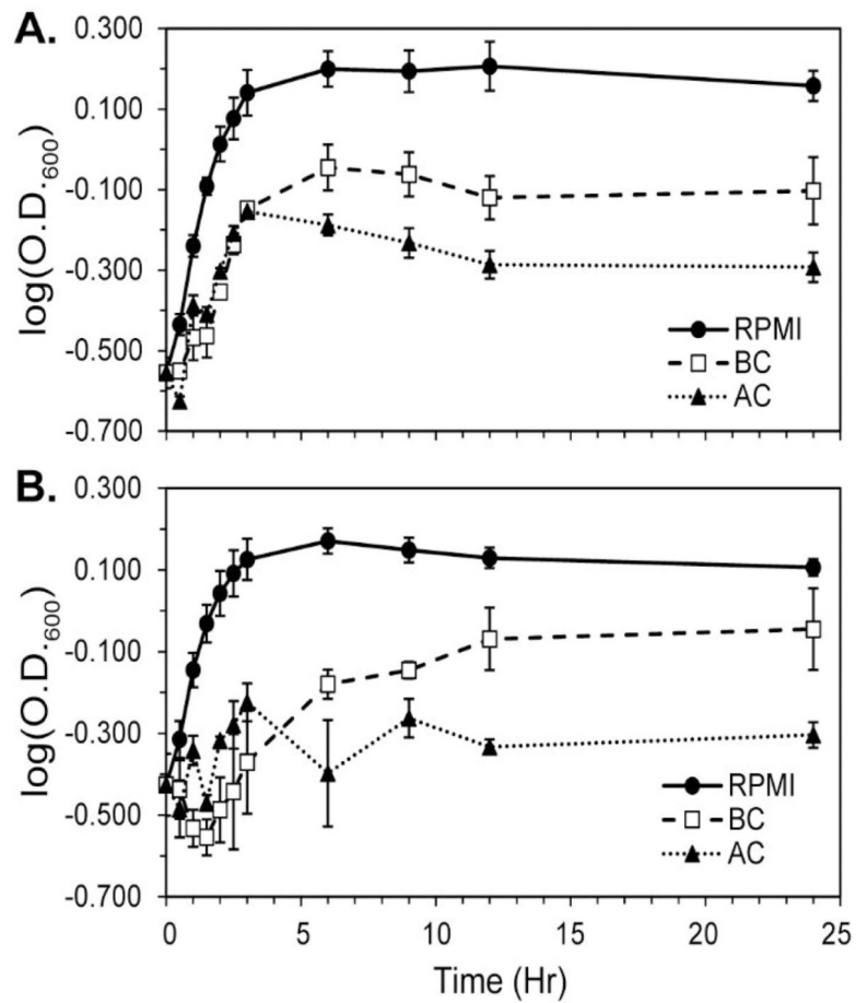
Figure 2. Growth curves of E. coli in RPMI Media.
