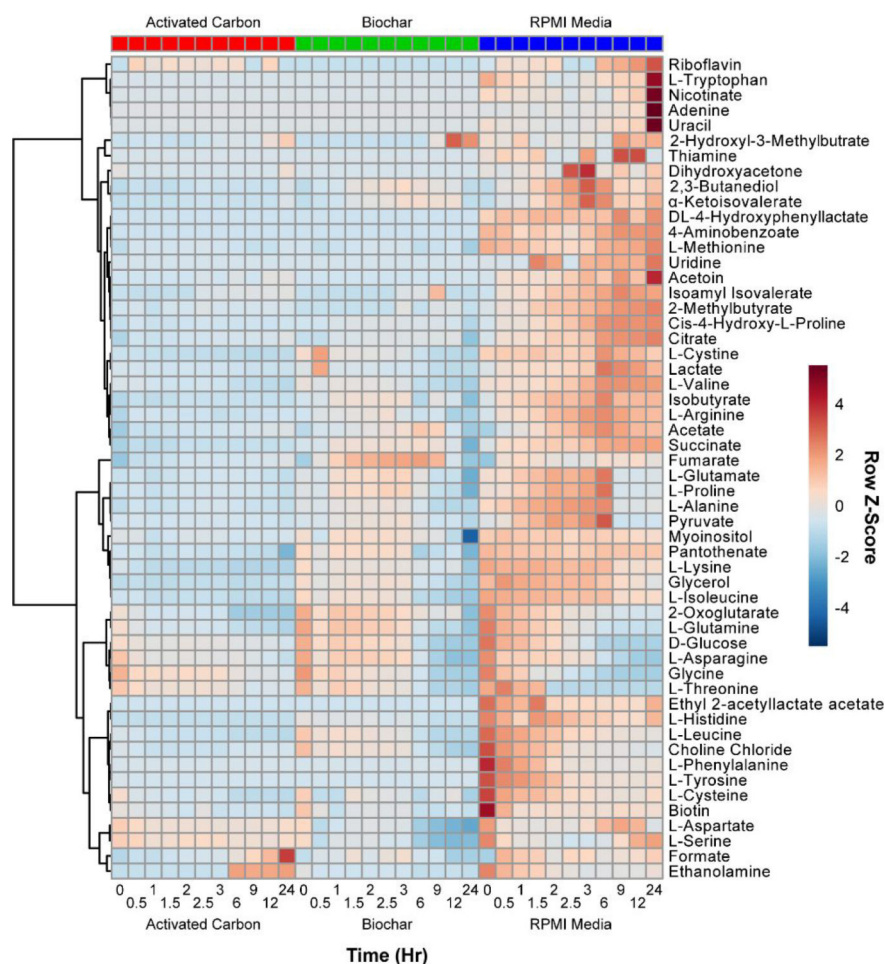
Figure 5. Heatmap of Extracellular Metabolites in Unfiltered Media.
