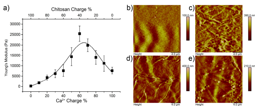
Figure 1. On the left a graph displaying the Young’s modulus dependent on the chitosan charge ratio (a); the line is added to guide the eye. Each point is an average of three measurements. On the right, representative AFM pictures of gels with a chitosan charge ratio of 0.0 (b), 0.2 (c), 0.4 (d), and 0.6 (e) are shown.
