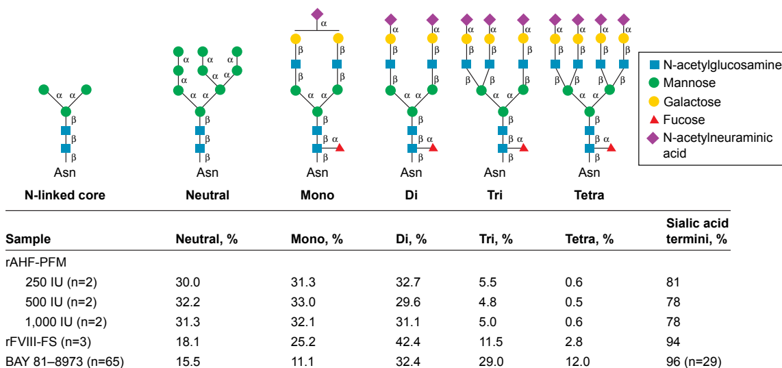
Figure 2 Glycan structures in BAY 81-8973, rFVIII-FS, and rAHF-PFM.
