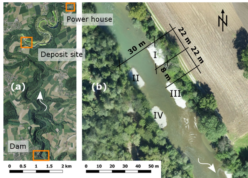
Figure 1. (a) Replenishment site and the locations of the dam and power house, background Geodata © swisstopo. (b) Configuration of the four sediment deposits in the Sarine River, background © Research unit Ecohydrology, ZHAW. The distance between the deposits was about a deposit length, the shift between the deposits on the left and the right bank is half a deposit length. The height of the deposits was ca. 1.5 m above the initial river-bed. The numbering refers to the name of the deposits from upstream to downstream: deposit I, II, III and IV.
