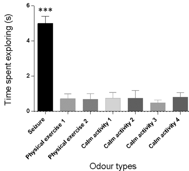
Figure 1. Mean time spent exploring (seconds) each odour type and 95% confidence intervals represented. (***) p < 0.001 ). Odour types were from a seizure ( seizure ), two from a sports session ( physical exercise 1 & 2 ), and four taken pseudo-randomly on different days during calm activity ( calm activity 1, 2, 3 & 4 ).
