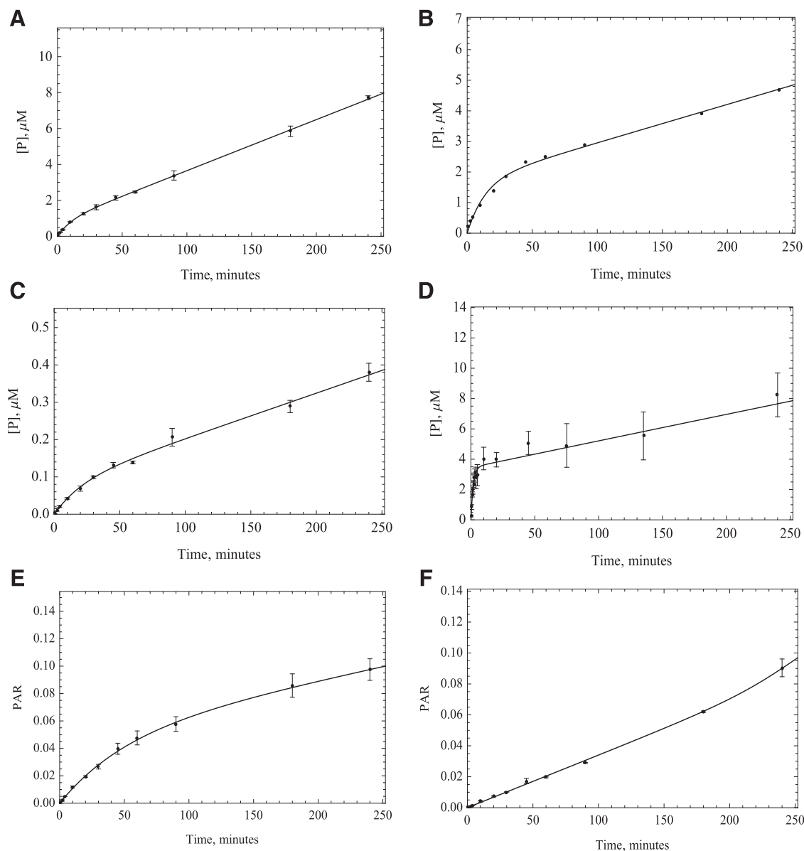
Fig. 2. Five times the K_m amount of the substrates: (A) O6BG, (B) DACA, (C) zaleplon, (D) phthalazine (E) BIBX1382, and (F) zonisipride were incubated with HLC ( 0.0051 \mu\text{M} AO) at 37^\circ\text{C} , and samples were quenched at different time points over 240 minutes ( n = 3 , P < 0.001 ). Data fitting was performed using the MAM. Based on the results, unlike the MM assumption, enzyme activity is not linear over time.
