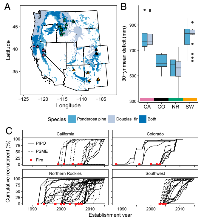
Fig. 2. Map of study site locations in the western United States (A), 30-y (1981–2010) mean climatic water deficit for sample sites within each region (B), and cumulative recruitment following fires for each site (C). Overall, 90 sites were sampled (see SI Appendix, Tables S1 and S2 for details). Ponderosa pine (PIPO) and Douglas-fir (PSME) ranges are shown in blue in A (72).
