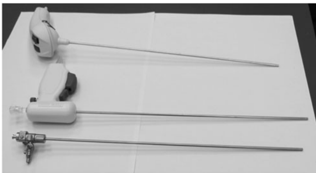
FIG. 1. Photo comparison of the three LSHP ( top to bottom : Lumenis Suction HP, Cook LithAssist, Storz LASER Suction Tube). LSHP = laser suction handpiece.
