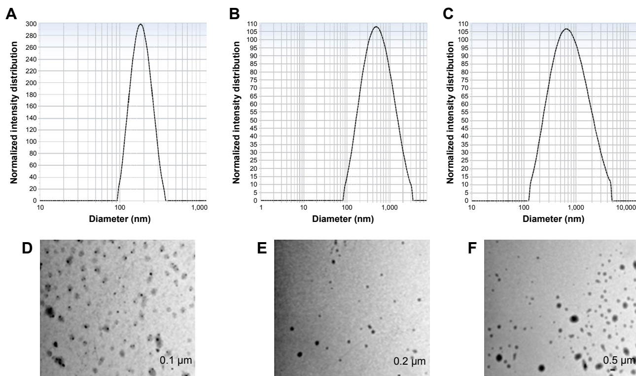
Figure 2 DLS measurement, nanoparticle size measurement of (A) PLGANP, (B) PLGA -GF NP, and (C) PLGA -GF -K4 NP and TEM images of (D) PLGANP, (E) PLGA -GF NP, and (F) PLGA -GF -K4 NP. Abbreviations: DLS, dynamic light scattering; GF, growth factor; NP, nanoparticle; PLGA, poly (lactic-co-glycolic acid).
