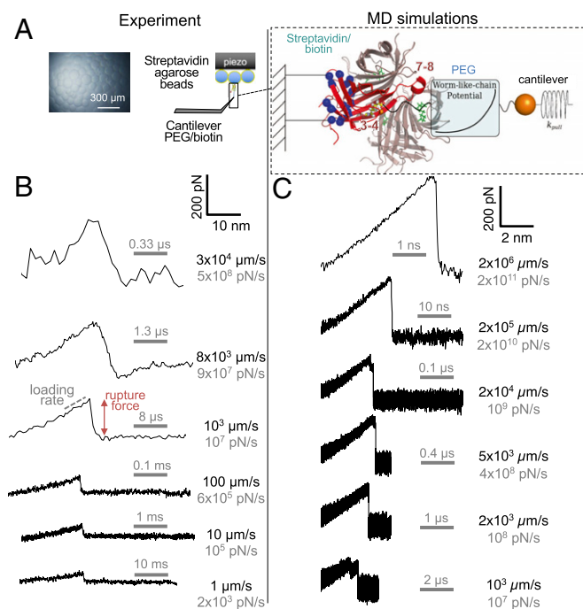
Fig. 1. High-speed and MD force spectroscopy of SA–b unbinding. ( A, Left ) HS-FS setup. SA agarose beads ( Top Left ) were immobilized on the sample surface while b was covalently attached to the microcantilever ( Bottom Left ) through a PEG linker (contour length \sim 10 nm). ( A, Right ) MD simulations setup and the SA–b tetramer used in the MD simulations with labeled loops 3–4 and 7–8 (PDB ID code 3RY2). ( B ) Experimental force–distance traces at velocities from 1 \mu\text{m/s} to 30,556 \mu\text{m/s} revealing bond rupture events using AC7 (top curve) and AC10 cantilevers (bottom curves). The stretching profile of the experimental curves was the result of stretching the PEG linker and deforming the agarose bead to which SA was linked. ( C ) Force–extension traces from the MD simulations at retraction velocities from 1,000 \mu\text{m/s} to 2 \times 10^6 \mu\text{m/s} .
