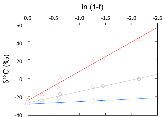
Fig. 2. Isotopic composition of bulk propane (gray diamonds), terminal position (blue circles), and central position (red triangles) of the remaining propane ( 1 - f ) during the course of anaerobic propane oxidation by the sulfate-reducing bacterium Desulfosarcina sp. strain Bu55. Fractionation factors ( \varepsilon , ‰) are calculated according to the slope of the line. \varepsilon_{\text{bulk}} = 12.8\text{‰} \pm 0.8\text{‰} ; \varepsilon_{\text{terminal}} = 2.8\text{‰} \pm 0.2\text{‰} ; \varepsilon_{\text{central}} = 33\text{‰} \pm 2\text{‰} . Error bars are smaller than the plotted symbols.
