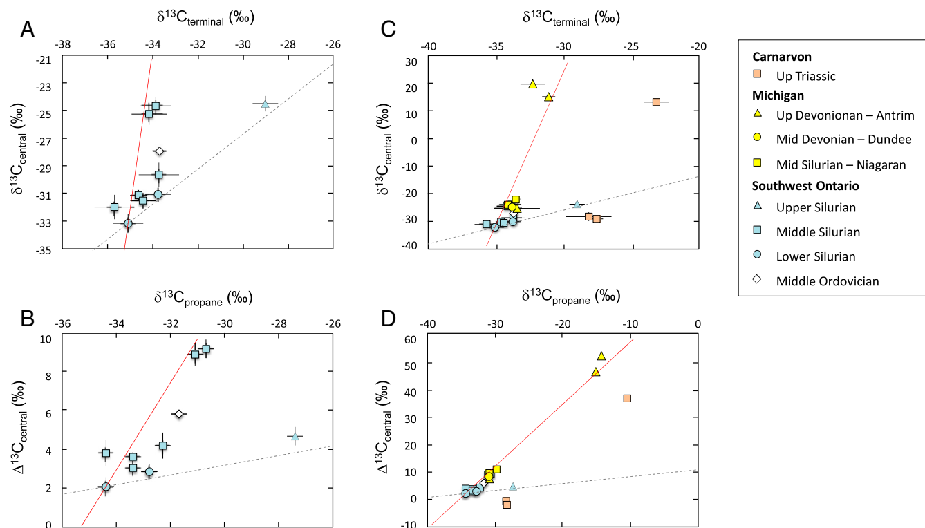
Fig. 3. Bulk ( \delta^{13}\text{C}_{\text{propane}} ) and position-specific carbon isotope composition of terminal ( \delta^{13}\text{C}_{\text{terminal}} ) and central ( \delta^{13}\text{C}_{\text{central}} ) positions of propane from Southern Ontario, Michigan, and Northern Carnarvon Basins. A and B show only data from Southwest Ontario, while C and D show the expanded scale and additional data from other basins. \Delta^{13}\text{C}_{\text{central}} is the relative ^{13}\text{C} enrichment at the central position ( \Delta^{13}\text{C}_{\text{central}} = \delta^{13}\text{C}_{\text{central}} - \delta^{13}\text{C}_{\text{terminal}} ). Lines are based on the slopes calculated from experiments and start from the propane sample with the lowest \delta^{13}\text{C} and \Delta^{13}\text{C}_{\text{central}} values. Red line: biodegradation trend identified in Fig. 1 A and B ; gray dotted line: thermogenic trend from cracking experiments of an n -alkane (yellow triangles in Fig. 1 A and B ). A and B are extended parts of C and D .
