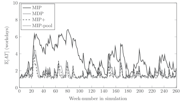
Figure 3. Week-dependent results for 5% cancellation.
