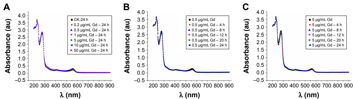
Figure S1 Ultraviolet-visible spectra results confirm that GON solution is very stable in RPMI 1640 medium. Notes: (A) Absorbance of GON with different concentrations after incubating at 37°C for 24 hours. (B, C) Absorbance of GON at concentrations 0.5 µg/mL (B) and 5.0 µg/mL (C) at various incubation time. Abbreviation: GONs, gadolinium oxide nanocrystals.
