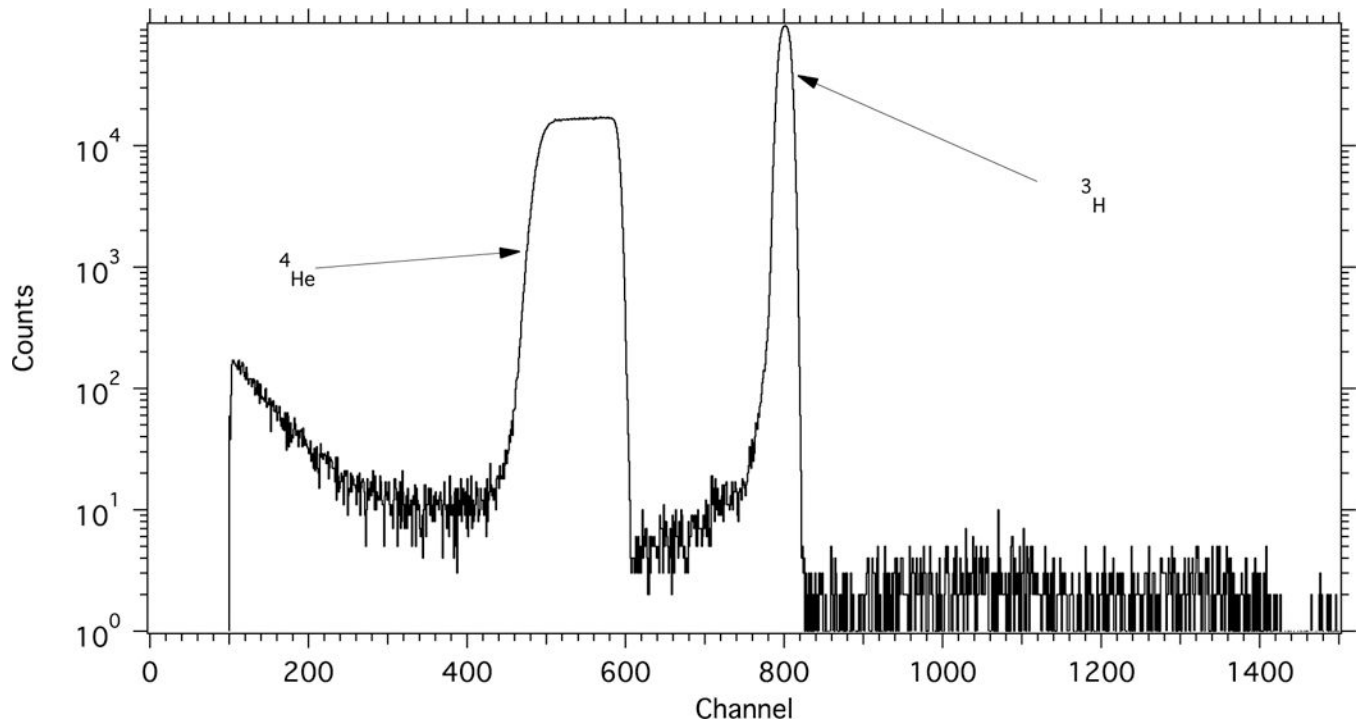
Figure 2. Typical pulse-height spectrum from ^6\text{Li} reaction products incident on a silicon detector in the neutron monitor.
