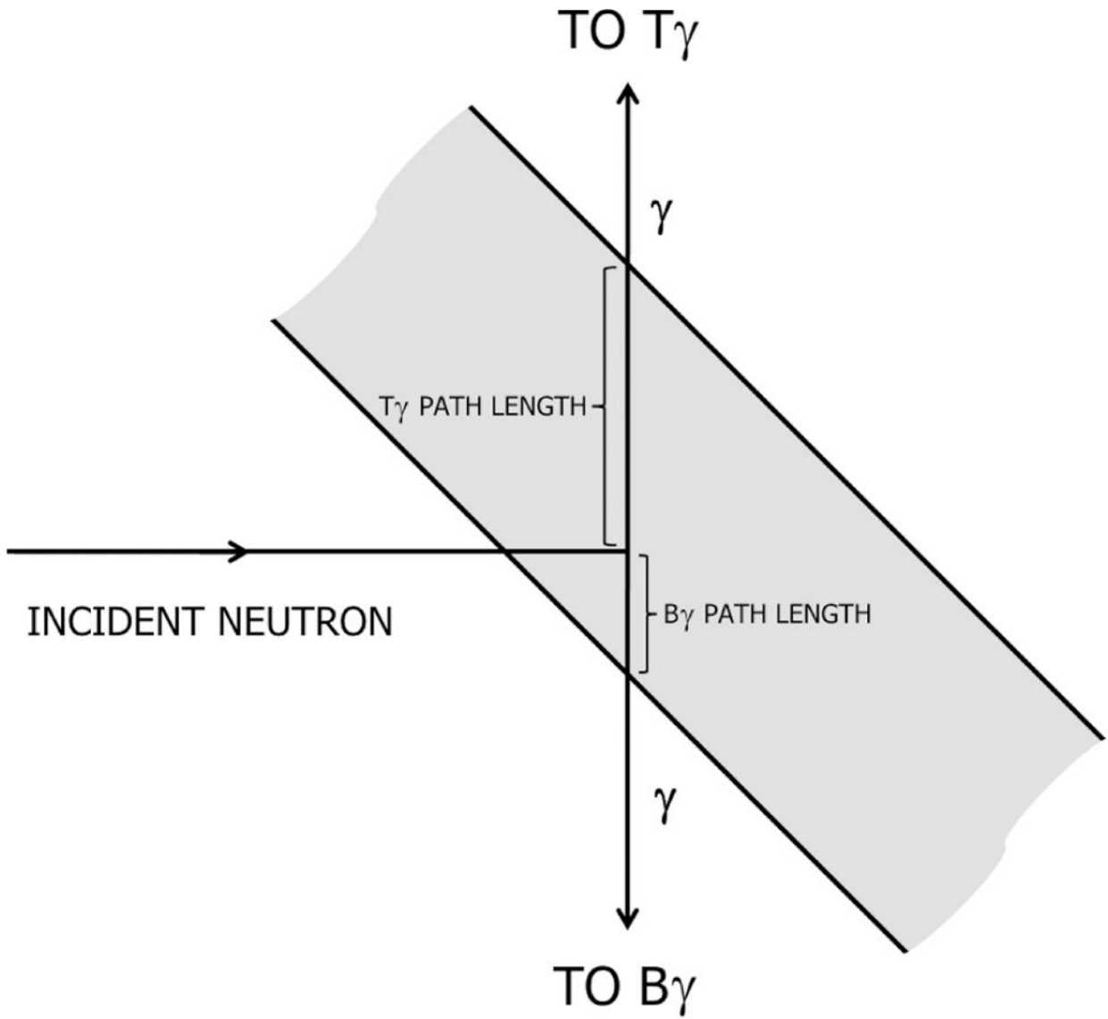
Figure 17. An illustration of the different path lengths through the thick target. The travel distance through the target to the bottom detector is greatly exaggerated.
