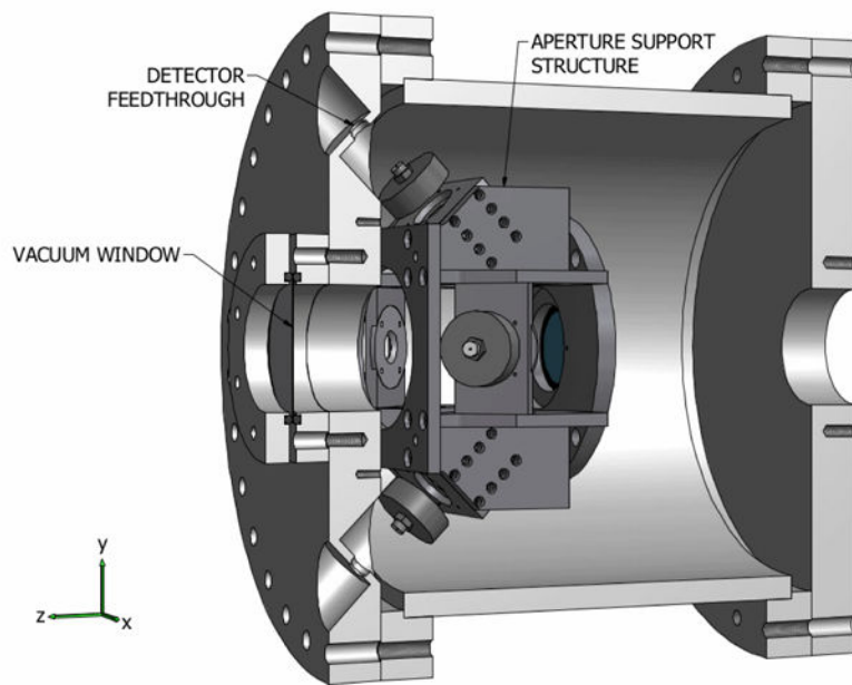
Figure 3. Illustrations of (a) a section view of the neutron monitor vacuum chamber and (b) a representation of the detection geometry.
