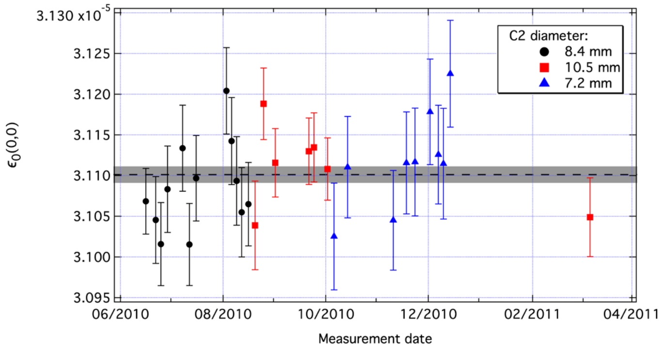
Figure 22. \epsilon_0(0,0) measurements for each of the three collimations. The dashed line is the weighted average of the values, and the gray band represents the \pm 1-\sigma region. The error bars represent statistical uncertainty only.
