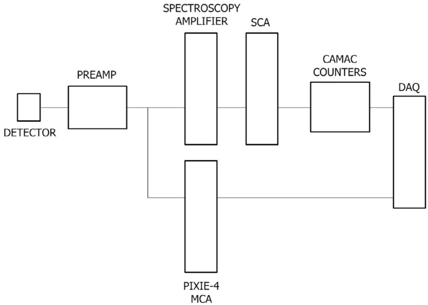
Figure 5. Block diagram of a detector's counting and spectroscopy electronics.
