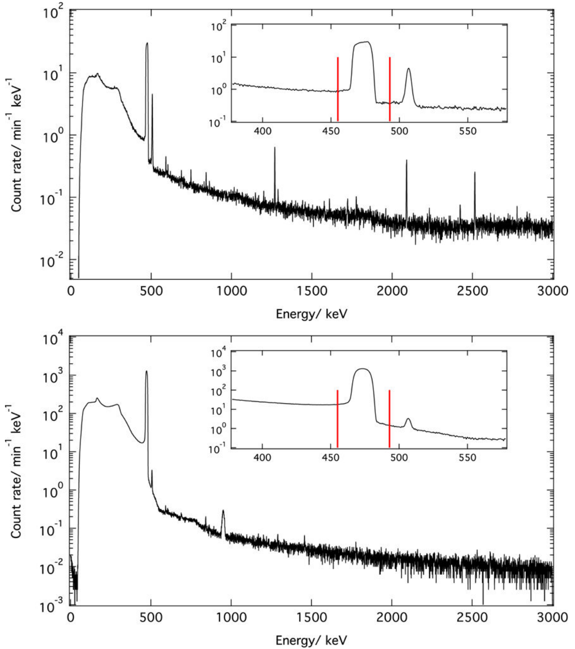
Figure 8. Top: plot of the gamma-ray spectrum from the thin 10 B target. The inset shows the region expanded around the 478 keV line, and the red lines indicate the analysis region. Bottom: plot of the gamma-ray spectrum from the thick 10 B target. The inset shows the region expanded around the 478 keV line, and the red lines indicate a typical analysis region.
