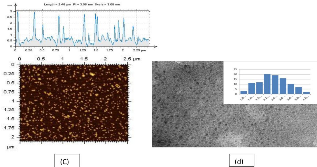
Figure 6: (a) AFM, (b) TEM topology images of free C-dots, (c) AFM and (d) TEM topology images of C-dots-transferrin-epirubicin-temozolomide (triple system) (C-DT). Scale bars in both the TEM images represent 10 nm. The carbon dot solutions were sonicated for 15 mins before the analysis.
