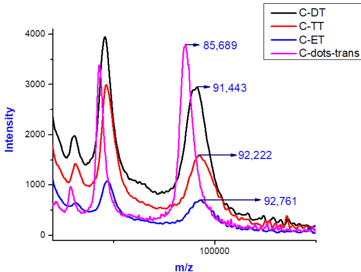
Figure 7: MALDI-TOF spectra of transferrin conjugated samples of C-dots-transferrin (C-dots-trans), C-dots-transferrin-epirubicin-temozolomide (C-DT) (triple system), C dots-transferrin-temozolomide (C-TT), and C-dots-transferrin-epirubicin (C-ET). Consistency of the data has been confirmed by the batch to batch analysis.
