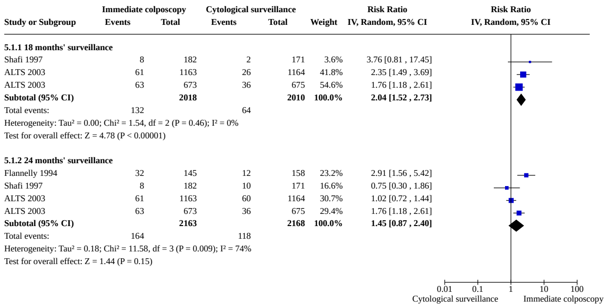
Figure 5. Forest plot of comparison: occurrence of CIN2 at different lengths of follow-up
