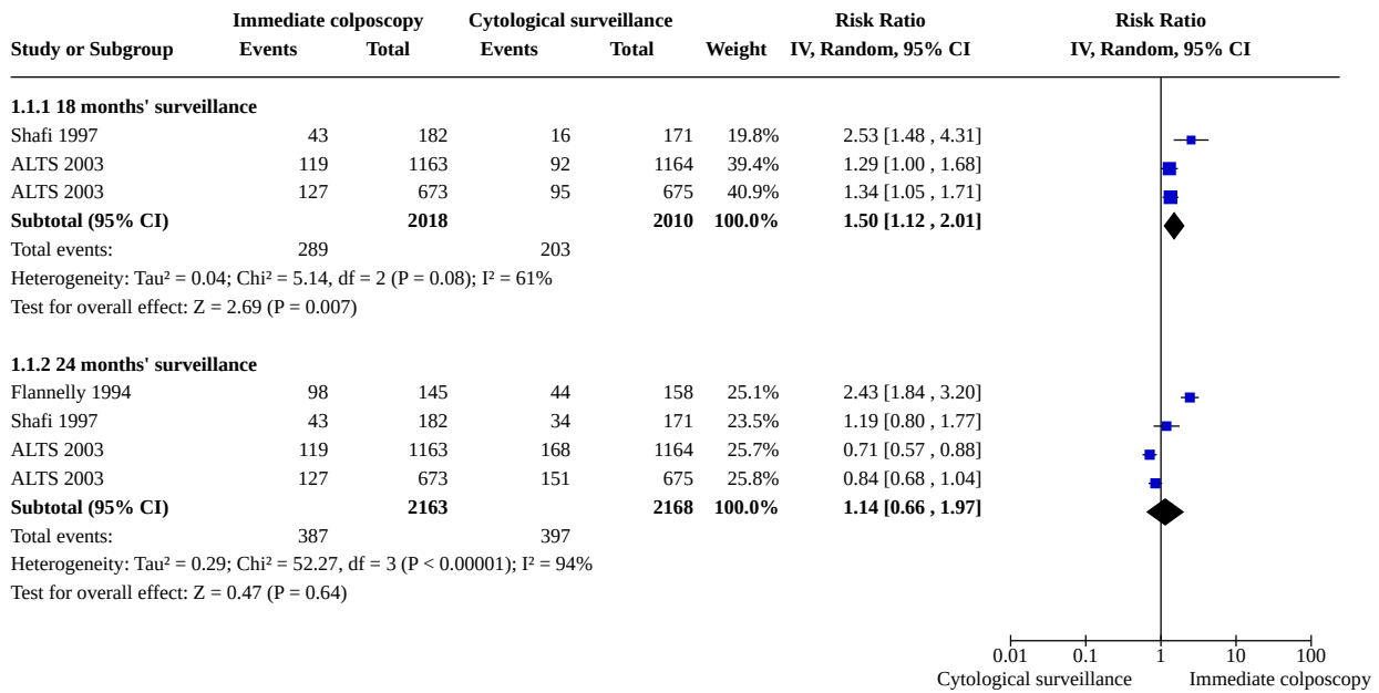
Figure 3. Forest plot of comparison: occurrence of CIN2+ at different lengths of follow-up
