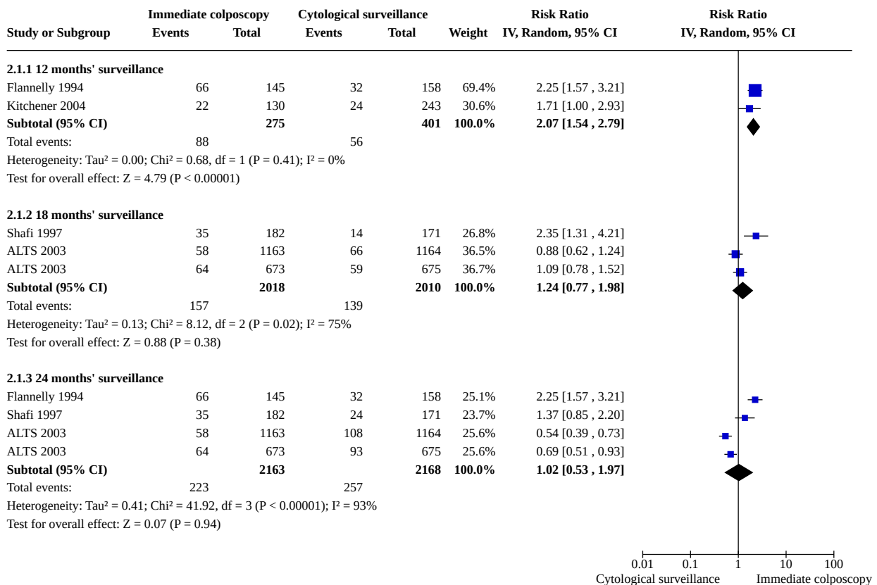
Figure 4. Forest plot of comparison: occurrence of CIN3+ at different lengths of follow-up
