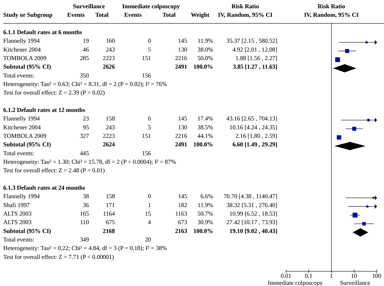
Figure 6. Forest plot of comparison: default rates at different lengths of follow-up
