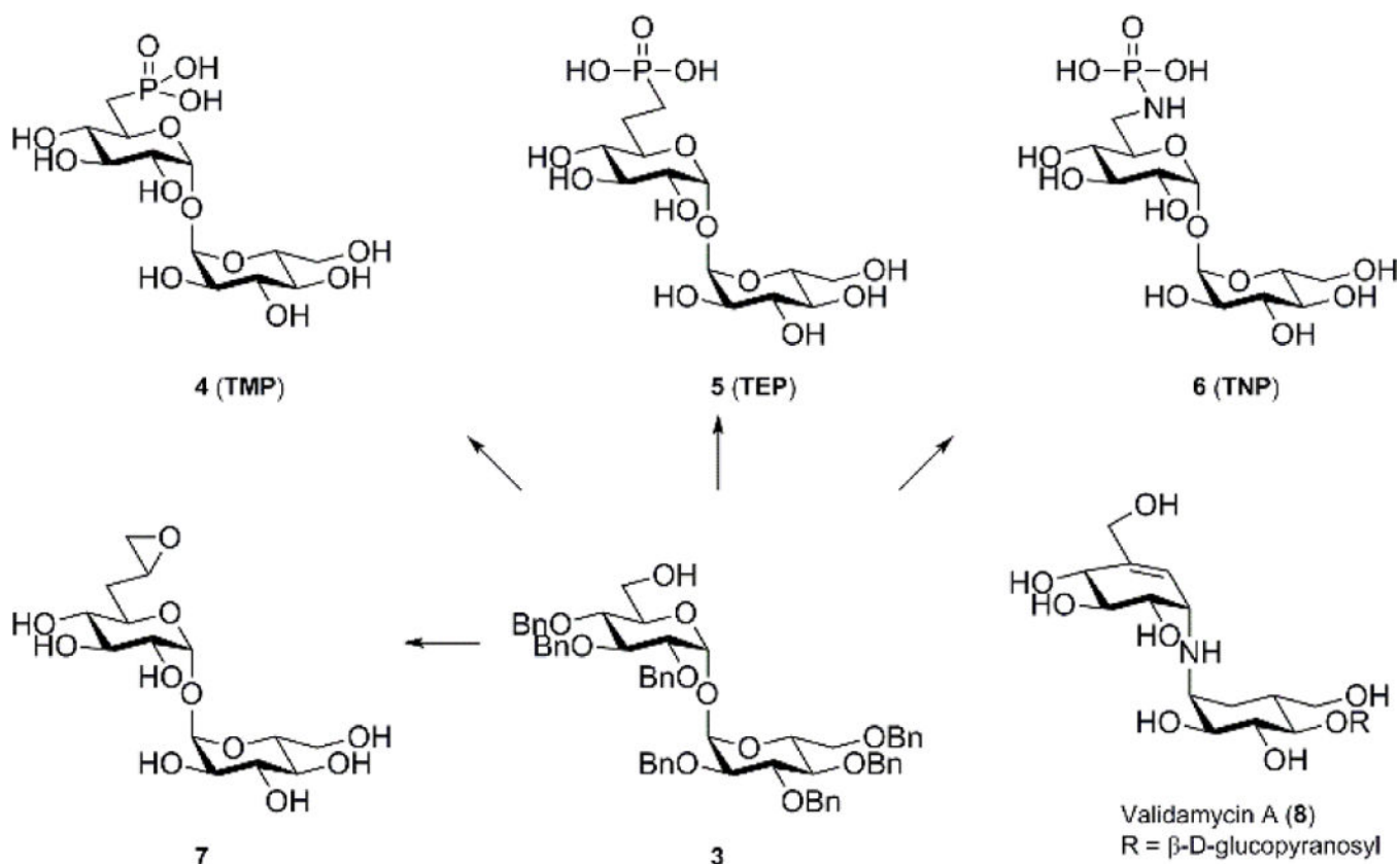
Figure 2. 6-deoxy- \alpha, \alpha' -trehalose derivatives prepared from heptabenzyl \alpha, \alpha' -trehalose derivative 3 and Validamycin A ( 8 ) which shows topological similarities with trehalose.
