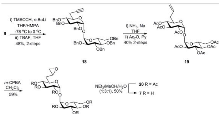
Scheme 4. Synthesis of 6-oxiranyl- \alpha,\alpha' -trehalose derivative 7 .
