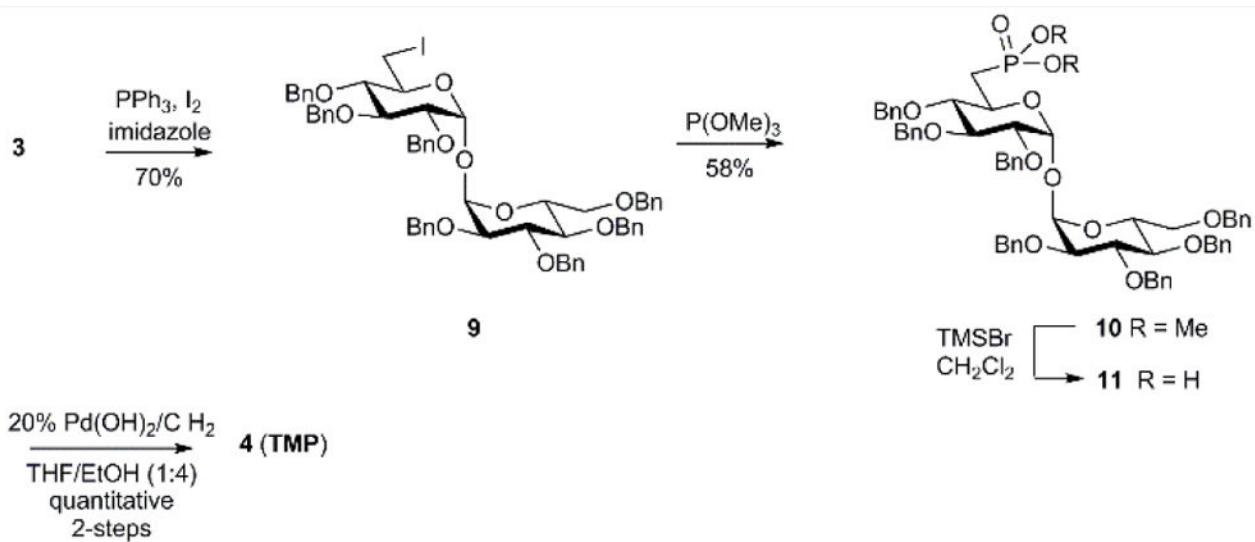
Scheme 1. Synthesis of 6-phosponic acid- \alpha,\alpha' -trehalose derivative TMP .
