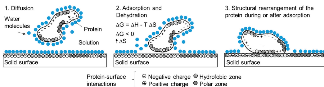
Figure 5. Adsorption process of a protein onto a solid surface [70,72,76].
