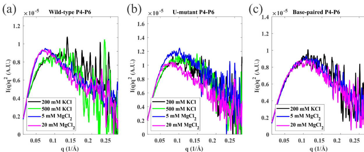
Figure 4: Kratky plots of SAXS data reporting the salt dependence of (a) wild-type P4-P6 (b) U-mutant P4-P6 and (c) base-paired P4-P6. These plots show a more pronounced peak when the molecule is in a more compact state. The wild-type P4-P6 shows two states, unfolded (black, green, showing no peak) in KCl and folded (blue, magenta, peak appears) in \text{MgCl}_2 respectively. The U-mutant P4-P6 appears unfolded in KCl, partially folded in 5 mM \text{MgCl}_2 and fully folded in 20 mM \text{MgCl}_2 . By design the base-paired P4-P6 remains unfolded across all the conditions.
