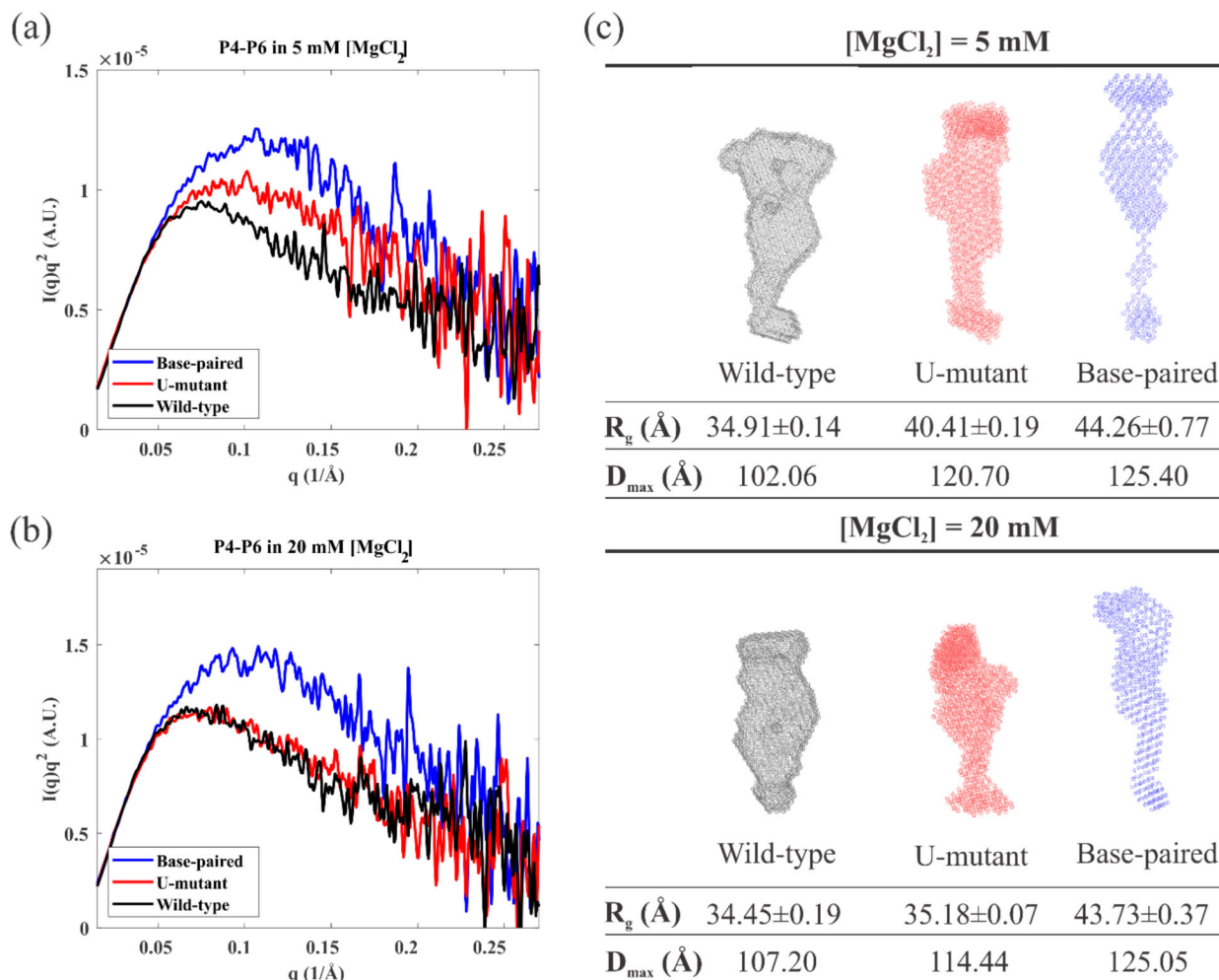
Figure 5: Comparison between the three different P4-P6 sequences in (a) 5mM MgCl 2 and (b) 20mM MgCl 2 . (c) The reconstructions of the SAXS profiles in 5mM and 20mM MgCl 2 (described in Material and Method section), color coded by the same scheme, assuming a homogeneous population. Global shape parameters are also reported.
