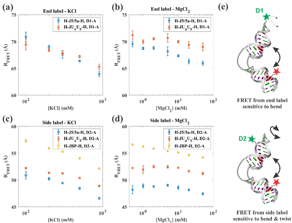
Figure 2: Measured effects on R_{FRET} as a function of KCl and MgCl 2 concentration for the D1-A (end-label) dye pair ((a) and (b)) and the D2-A (side-label) dye pair ((c) and (d)). Data for all three constructs are shown: H-J5/5a-H (blue), H-JU 4 U 5 -H (red) and H-JBP-H (orange). The error bars represent the combination of the 95% confidence interval of the fit parameter and the standard deviations of at least two independent measurements. Part (e) shows a cartoon representing the RNA junction constructs and the associated label positions. The D1 label is closer to the helical axis and is more sensitive to overall bend angle, while the D2 label is off-axis and sensitive to both bending and relative twisting.
