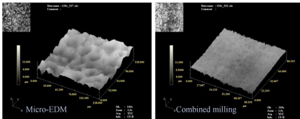
Figure 22. SR of the bottom surface [171].
