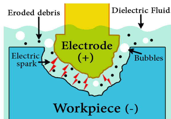
Figure 2. Principle of EDM.
