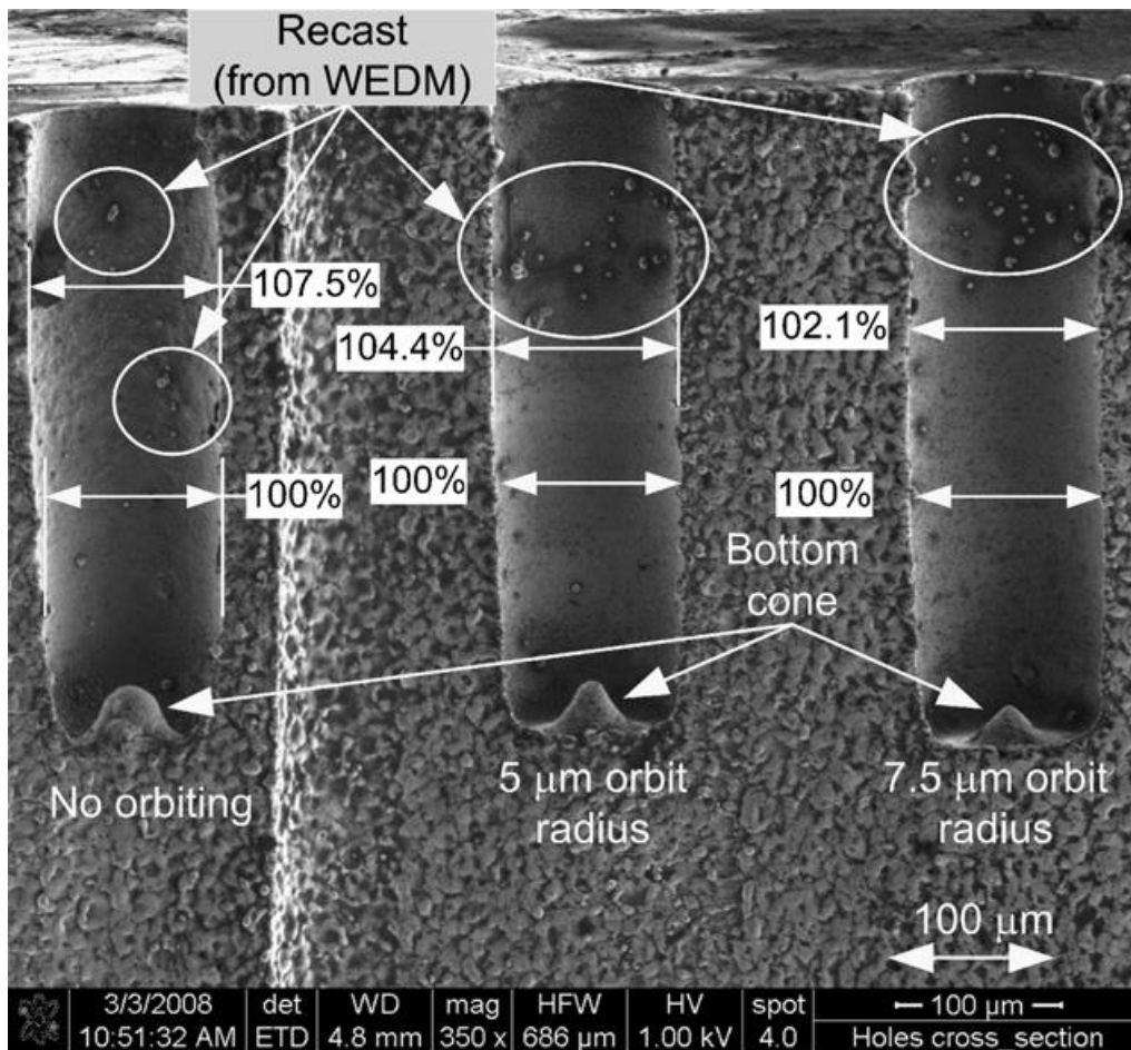
Figure 20. Cross-section of 500 µm deep micro-holes without orbiting; with 5 µm orbit radius; and with 7.5 µm orbit radius drilled with 60 V and 47 pF capacitance [182].
