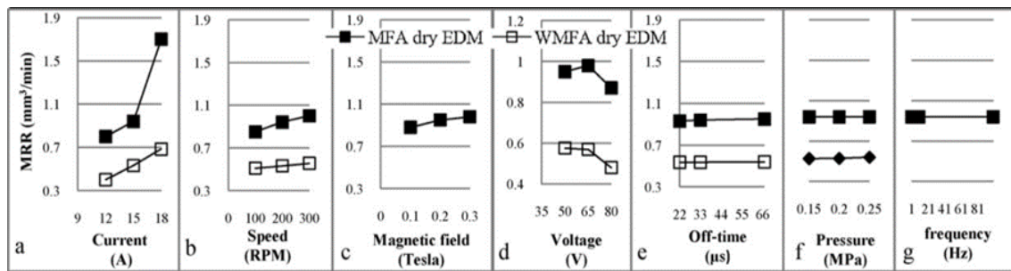
Figure 24. Comparative parametric plots for the MRR in MFA dry EDM and WMFA dry EDM [136].
