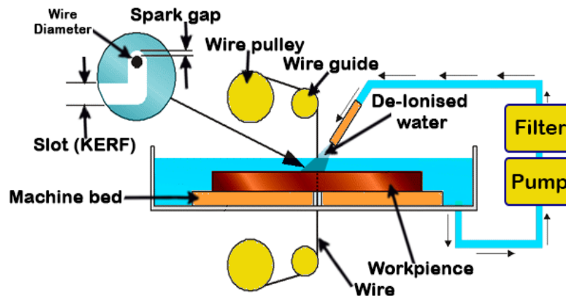
Figure 4. Schematic diagram of the wire EDM.
