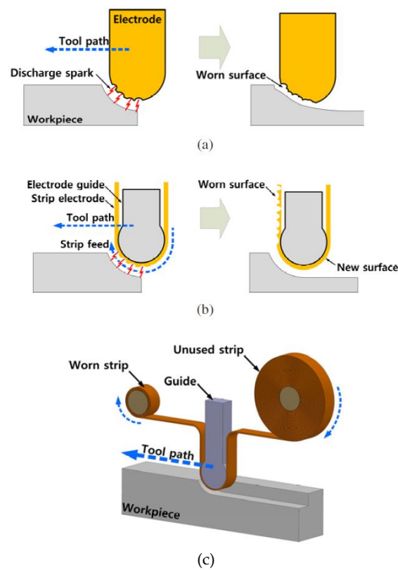
Figure 16. (a) General EDM; (b) strip EDM; and (c) concept of the strip EDM [159].
