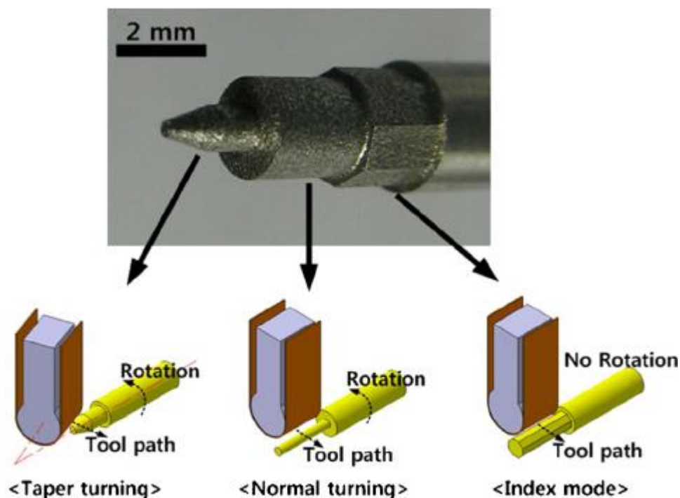
Figure 18. Product created using three kinds of strip-EDM turning [166].
