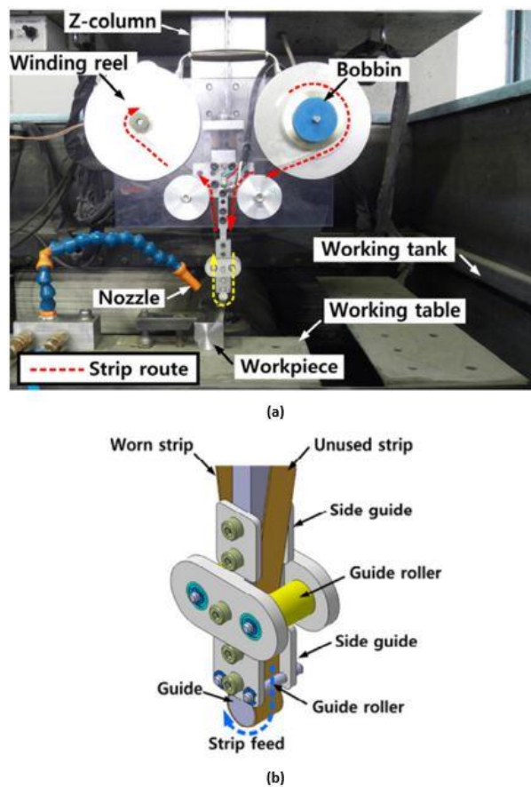
Figure 15. (a) Strip-EDM system; and (b) electrode guide [159].
