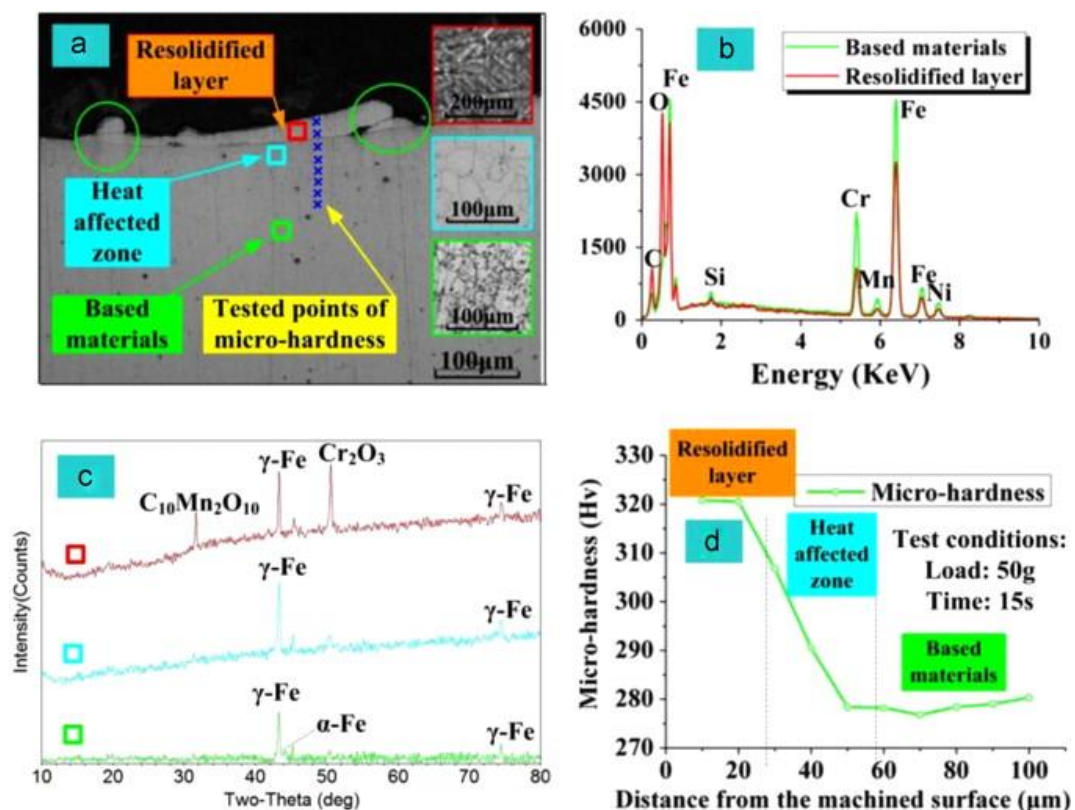
Figure 6. (a) Scanning Capacitance Microscopy (SCM) photograph of the cross-section of the AISI304 in high-speed dry EDM; (b) EDS spectra of the re-solidified layer and base materials; (c) XRD diffractograms of the re-solidified layer, heat affected zone and base materials; and (d) micro-hardness of the cross-section [48].
