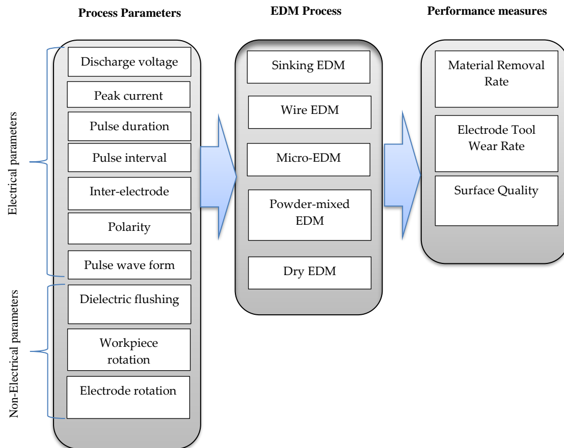
Figure 1. Electric discharge machining (EDM) processes, process parameters and performance measures.
