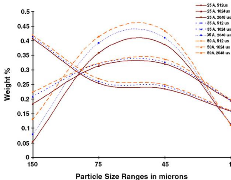
Figure 14. Particle size distributions in deionized water with varying current intensities and pulse widths [170].
