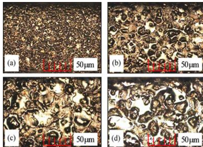
Figure 27. The surface roughness caused by various peak currents: (a) 1.5 A (0.715 \mu\text{m} ), (b) 3 A (0.796 \mu\text{m} ), (c) 5 A (0.855 \mu\text{m} ) and (d) 6 A (0.994 \mu\text{m} ) [187].
