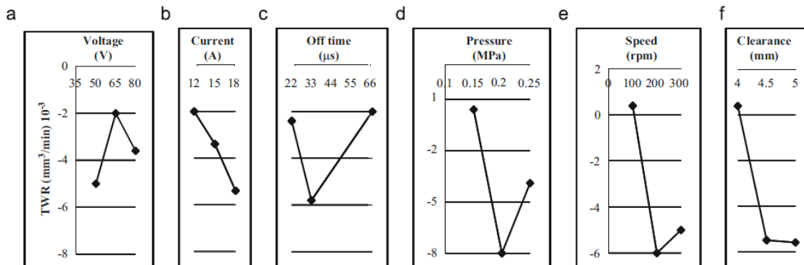
Figure 12. (a–f) Main effects of input parameters associated with the tool wear rate (TWR) [174].
