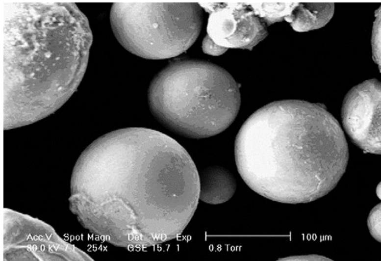
Figure 13. Scanning electron micrograph of particles produced in water at 50 A and 512 ms [170].
