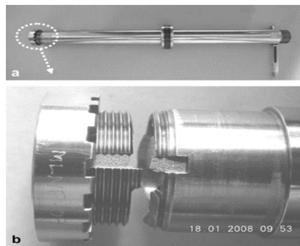
Figure 26. Photographs showing (a) the failed piston and (b) the location of failure [195].
