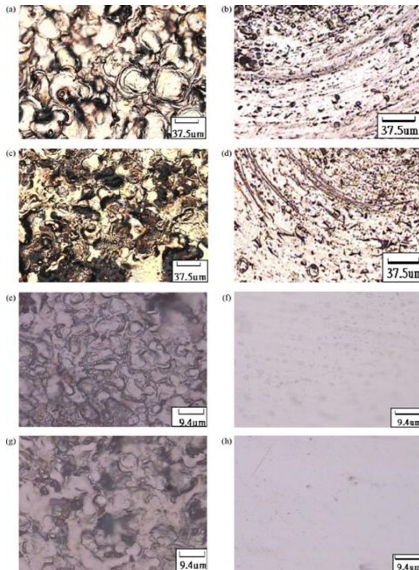
Figure 29. The machined surface for different concentrations of starch and abrasive \text{Al}_2\text{O}_3 , under discharge capacitances of 0.068 \mu\text{F} and 0.01 \mu\text{F} : (a) 10 wt.% starch without \text{Al}_2\text{O}_3 , \text{SR} = 1.24 \mu\text{m} C = 0.068 \mu\text{F} ; (b) 10 wt.% starch - 10 wt.% \text{Al}_2\text{O}_3 , \text{SR} = 0.26 \mu\text{m} C = 0.068 \mu\text{F} ; (c) 20 wt.% starch without \text{Al}_2\text{O}_3 , \text{SR} = 1.12 \mu\text{m} C = 0.068 \mu\text{F} ; (d) 20 wt.% starch-10 wt.% \text{Al}_2\text{O}_3 , \text{SR} = 0.14 \mu\text{m} C = 0.068 \mu\text{F} ; (e) 10 wt.% starch without \text{Al}_2\text{O}_3 , \text{SR} = 0.52 \mu\text{m} C = 0.01 \mu\text{F} ; (f) 10 wt.% starch-10 wt.% \text{Al}_2\text{O}_3 , \text{SR} = 0.06 \mu\text{m} C = 0.01 \mu\text{F} ; (g) 20 wt.% starch without \text{Al}_2\text{O}_3 , \text{SR} = 0.46 \mu\text{m} C = 0.01 \mu\text{F} ; and (h) 20 wt.% starch-10 wt.% \text{Al}_2\text{O}_3 , \text{SR} = 0.08 \mu\text{m} C = 0.01 \mu\text{F} [88].
