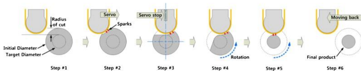
Figure 17. Strip-EDM turning process [166].
