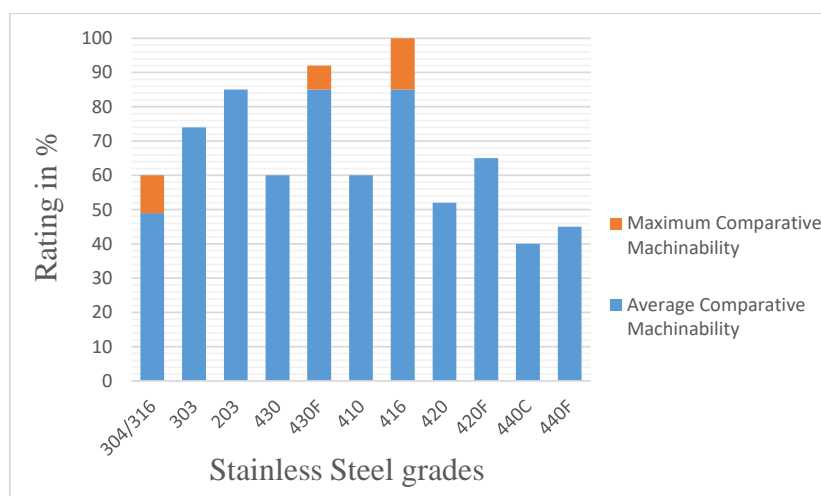
Figure 5. Comparative machinability of frequently used stainless steels and their free-machining counterparts.
