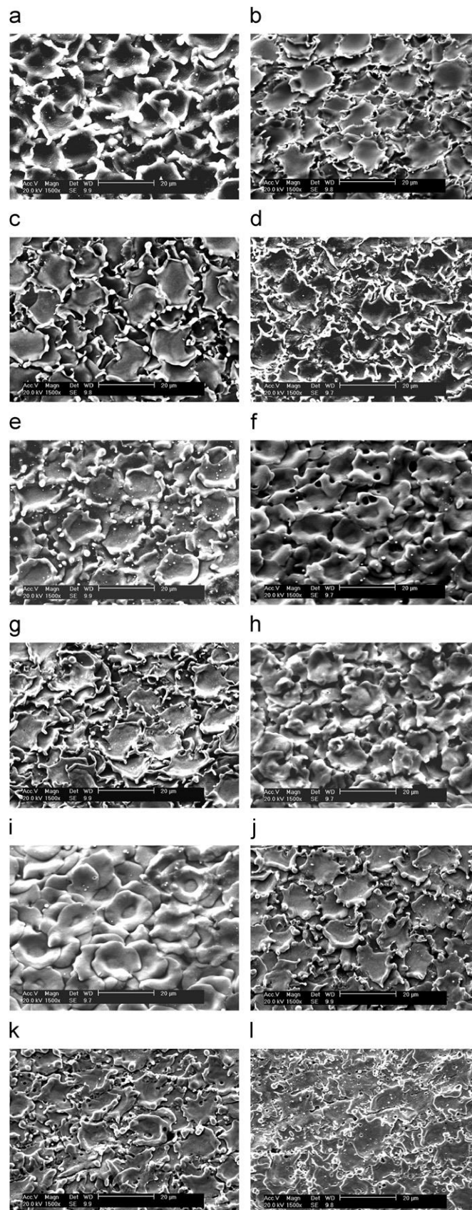
Figure 30. SEM images of the discharge craters for different workpiece materials: (a) aluminium (Al), (b) silver (Ag), (c) brass (Br), (d) copper (Cu), (e) nickel (Ni), (f) steel (Fe), (g) platinum (Pt), (h) titanium (Ti), (i) stainless steel, (j) tantalum (Ta), (k) molybdenum (Mo) and (l) tungsten (W) [203].
