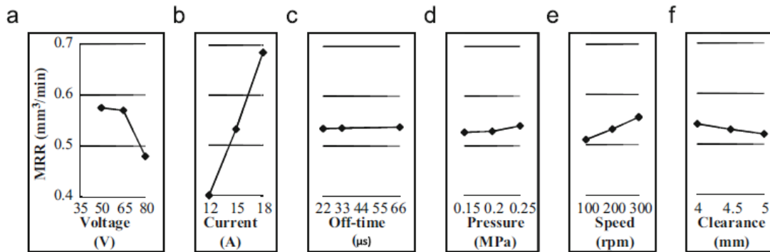
Figure 11. (a–f) Main effects of the input parameters associated with the MRR [174].
