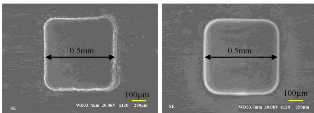
Figure 23. Scanning electron microscope (SEM) photos of the square cavity machined by EDM and micro-EDM combined with milling [171].
