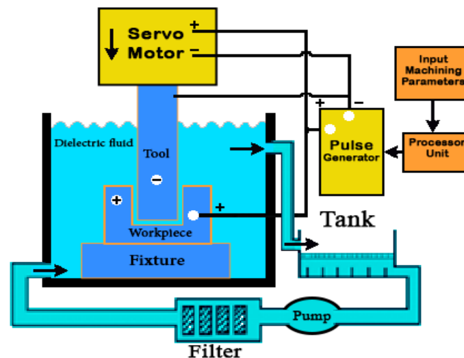
Figure 3. Schematic diagram of the die-sinking EDM.
