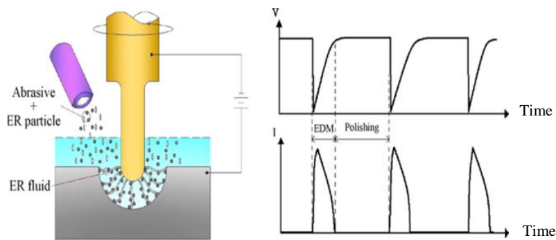
Figure 28. Schematic diagram of the proposed method using the ER fluid and abrasive grit [88].
