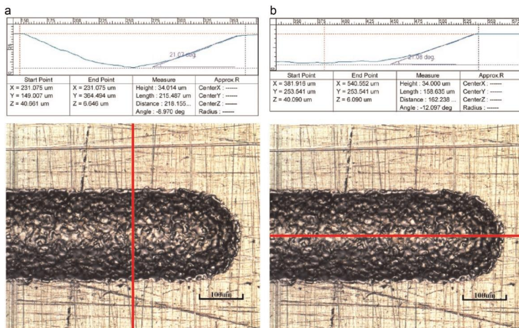
Figure 31. Actual machined results for the workpiece under Zeiss confocal microscope when the layer thickness is 43.5 µm: (a) cross section and (b) longitude section [197].
