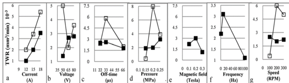
Figure 25. Comparative parametric plots for the TWR in MFA dry EDM and WMFA dry EDM [136].
