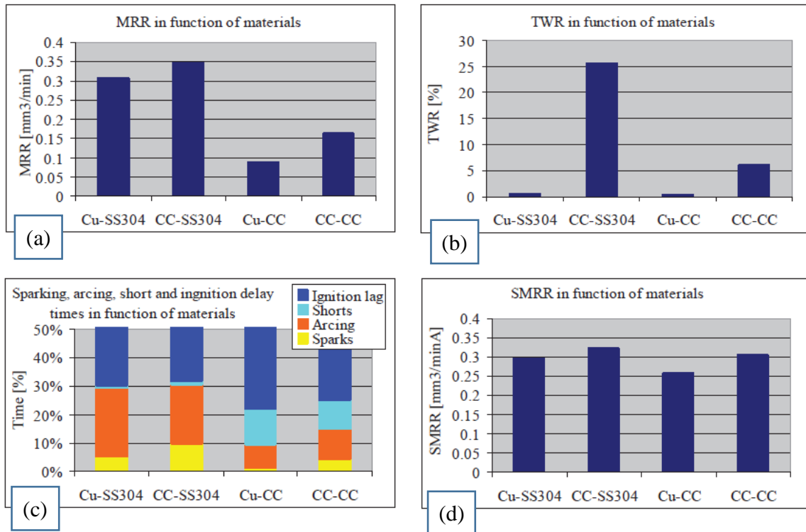
Figure 10. (a) MRR dependence on anode and cathode material combinations; (b) TWR as a function of anode and cathode material combinations; (c) sparking, arcing, shorts and ignition delay times as a function of anode and cathode material combinations; and (d) current specific MRR as a function of the anode and cathode material combinations [176].
