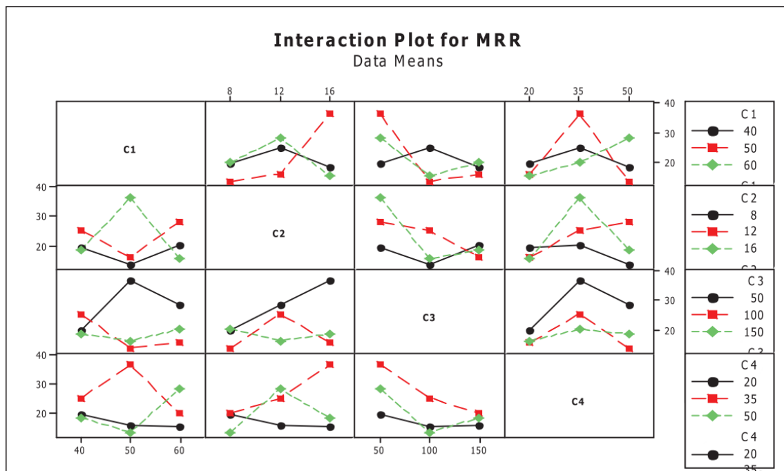
Figure 9. Interaction plot of the material removal rate (MRR) [157].
