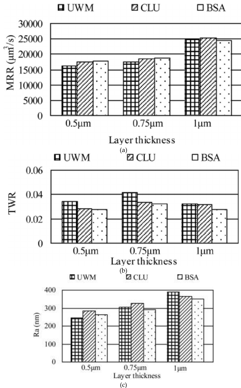
Figure 21. (a) MRRs for the three methods UWM, CLU and BSA; (b) TWRs for the three methods; and (c) SR for the three methods [167].
