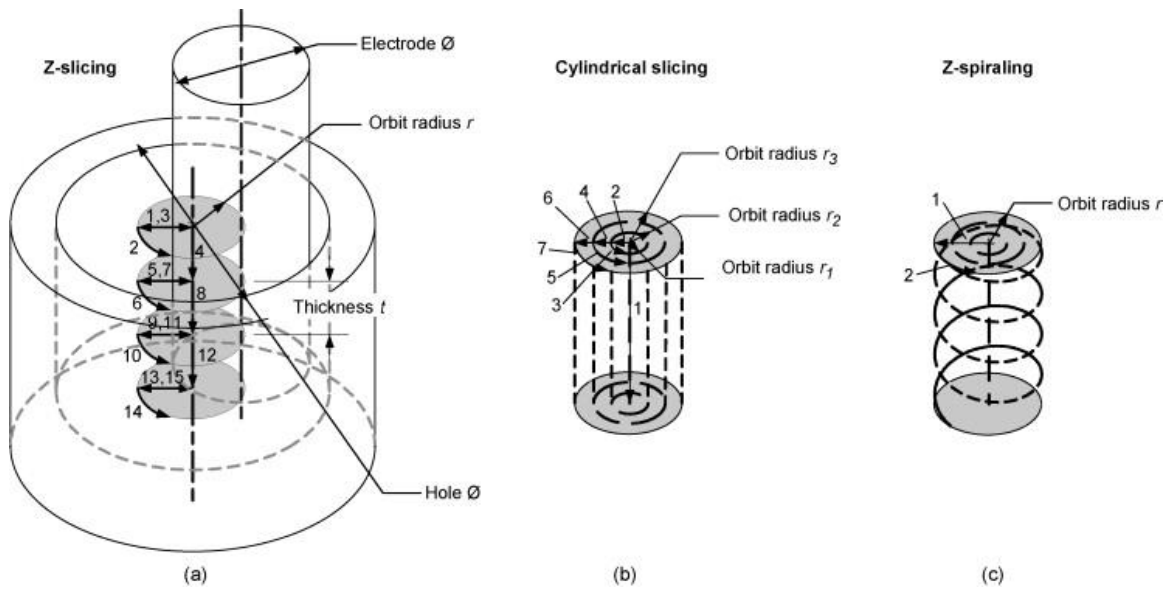
Figure 19. Electrode orbiting strategies: (a) slicing the hole into cylinders of thickness t and radius r ; (b) slicing the hole into cylindrical shells of radius r ; and (c) spiralling into the hole with radius r [182].
