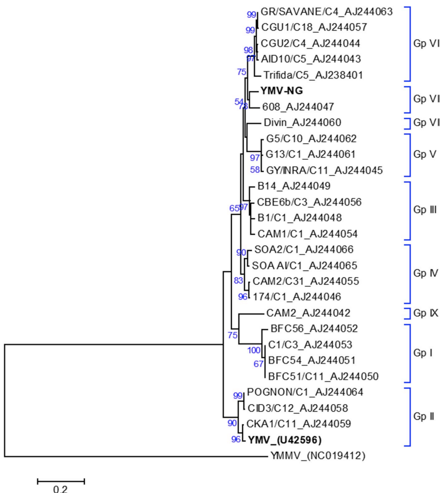
Fig. 7. Molecular phylogenetic analysis of the Nib-CP-3'-UTR region of YMV-NG (GenBank accession number MG711313) in comparison to 26 YMV sequences and their group assignments from a phylogenetic analysis by Bousalem et al. [62]. Yam mild mosaic virus (YMMV) was used as an outgroup. The sequences were aligned using the CLUSTALW tool, and the evolutionary relationships were inferred using the maximum-likelihood method based on the Hasegawa–Kishino–Yano model [65], conducted in MEGA7 [63]. Bootstrap analysis was performed with 1000 replicates and the cut-off value was 50%. The tree is drawn to scale, with branch lengths reflecting the number of substitutions per site.
