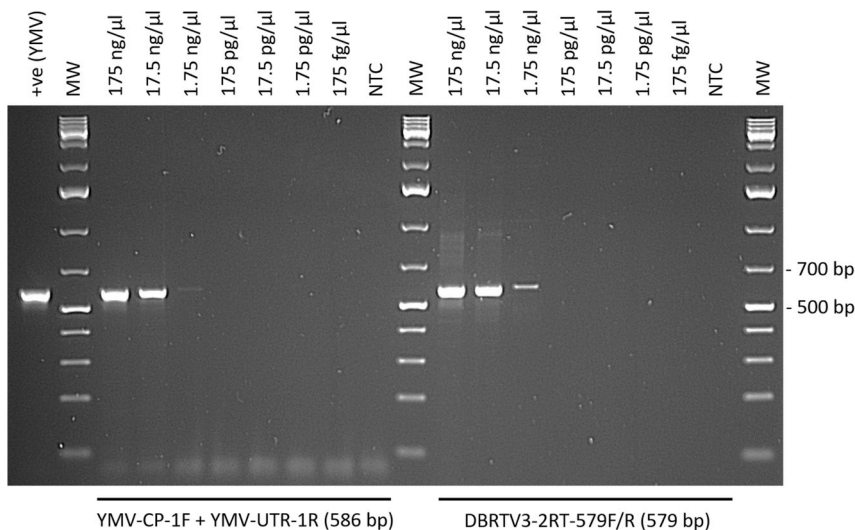
Fig. 8. Sensitivity of one-step RT-PCR assay for the detection of YMV and DBRTV3-[2 R T] in 10-fold serially diluted total RNA from yam landrace Makakusa used for RNA-seq virus detection. MW: GeneRuler™ 1 kb Plus DNA Ladder (Thermo Scientific, UK); NTC: non-template (water) control; +ve (YMV): positive control for YMV (RNA of a YMV infected yam plant detected using the one-step RT-PCR assay described in Silva et al. [51]).
