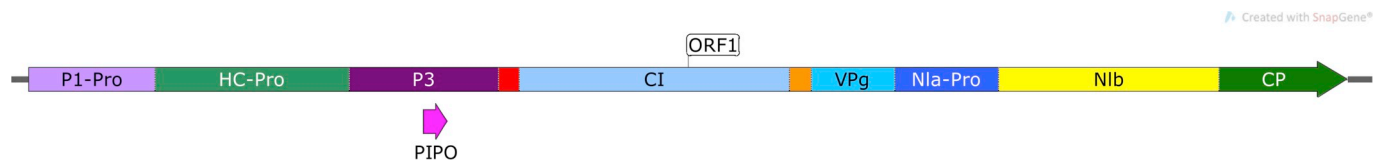
Fig. 6. Linear representation of the genome of YMV Nigeria isolate (YMV-NG, GenBank accession number MG711313), showing P1-Pro, protein 1 protease; HC-Pro, helper component protease; P3, protein 3; PIPO, pretty interesting Potyviridae ORF; 6K1, 6-kDa peptide (red); CI, cytoplasmic inclusion; 6K2, 6-kDa peptide (orange); VPg, viral protein genome-linked; NIa-Pro, nuclear inclusion A protease; NIB, nuclear inclusion B RNA-dependent RNA polymerase; and CP, coat protein, according to Wylie et al. [74].
