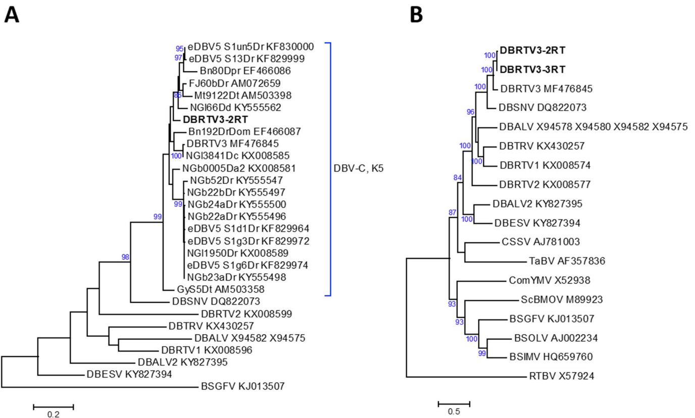
Fig. 5. Molecular phylogenetic analysis of new members of the species Dioscorea bacilliform virus (DBV) belonging to the genus Badnavirus . Bootstrap consensus phylogenetic trees were constructed based on 528-bp partial nucleotide sequences of the badnavirus RT-RNaseH domain (A) or on full-length nucleotide sequences of the genomes of DBVs and other badnavirus type members (B). The partial RT-RNaseH sequences of eight DBV genomes and all yam badnavirus sequences with nucleotide sequence identity values above 80% relative to DBRTV3-[2RT] in similarity searches with the NCBI BLAST and consequently belonging to monophyletic species group K5 described by Kenyon et al. [24] were included in the tree presented in (A), and Banana streak GF virus (BSGFV) was used as an outgroup. Rice tungro bacilliform virus (RTBV) functioned as an outgroup in (B). GenBank accession numbers are provided, and DBRTV3-[2RT] (GenBank accession number MG711311) and DBRTV3-[3RT] (GenBank accession number MG711312) are highlighted in bold. The partial RT-RNaseH sequences of DBRTV3-[2RT] and DBRTV3-[3RT] are identical and only DBRTV3-[2RT] was included in the tree shown in (A). Alignments of partial RT-RNaseH sequences were performed in MEGA7 [63] using the CLUSTALW tool, and full genome alignments were done using MAFFT [64]. Evolutionary relationships were inferred using the maximum-likelihood method based on the Hasegawa–Kishino–Yano model [65], conducted in MEGA7. Bootstrap analysis was performed with 1000 replicates and the cut-off value was 80%. The trees are drawn to scale, with branch lengths measured in the number of substitutions per site.
