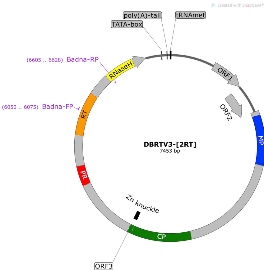
Fig. 4. Circular representation of the Dioscorea bacilliform RT virus, isolate DBRTV3-[2RT] (GenBank accession number MG711311) genome organisation, showing the tRNA Met -binding site; the TATA-box; the putative poly(A) tail; open reading frame (ORF)1; ORF2; ORF3 containing putative movement protein (MP), capsid protein zinc-finger domain (CP and Zn knuckle), pepsin-like aspartate protease (PR), reverse transcriptase (RT) and RNaseH conserved motifs; and binding sites for Badna-FP/-RP primers (purple) [73], which amplify a 579-bp fragment of the RT-RNaseH domain and are used for taxonomic assessment of badnaviruses [19].
