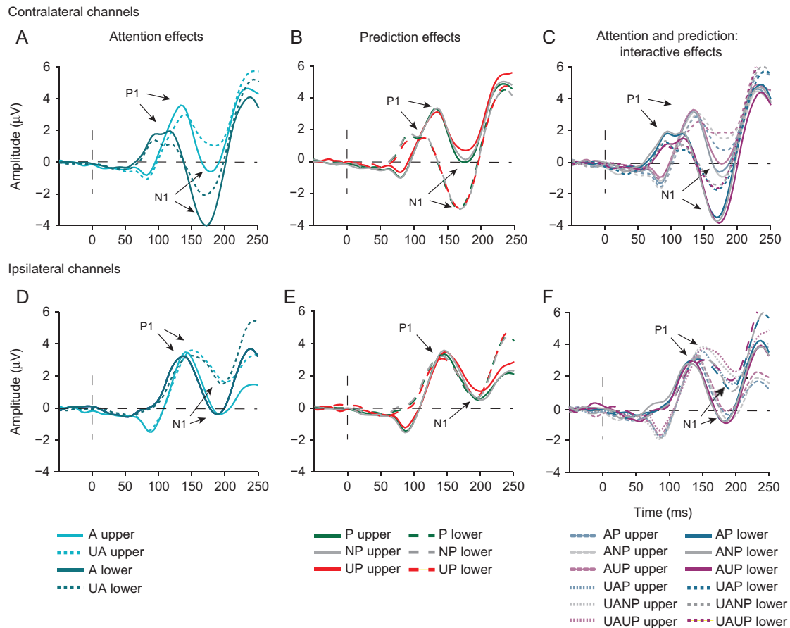
Figure 7. Effects of attention and prediction on later stages of visual information processing indexed by the P1 and N1 ERP components. (A, D) Attention was also associated with a larger contralateral P1 and bilateral N1. (B, E) Predictions did not modulate P1 and N1 amplitudes. (C, F) Prediction did marginally modulate the N1 peak in interaction with attention.
