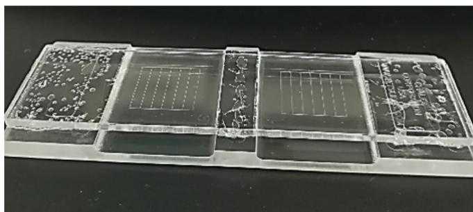
Figure 5. Two-chamber McMaster counting slide. 0.15 cm depth; 1 cm 2 .
