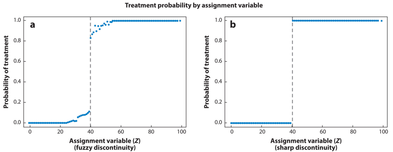
Figure 2. Probability of receiving treatment in fuzzy and sharp regression discontinuity designs. (a) A fuzzy regression discontinuity: probability of treatment changes gradually at values of the assignment variable close to the cutoff. (b) A sharp regression discontinuity: probability of treatment changes from 0 to 1 at the cutoff. Source: Reproduced from Moscoe (2015) (57) with permission from Elsevier.
