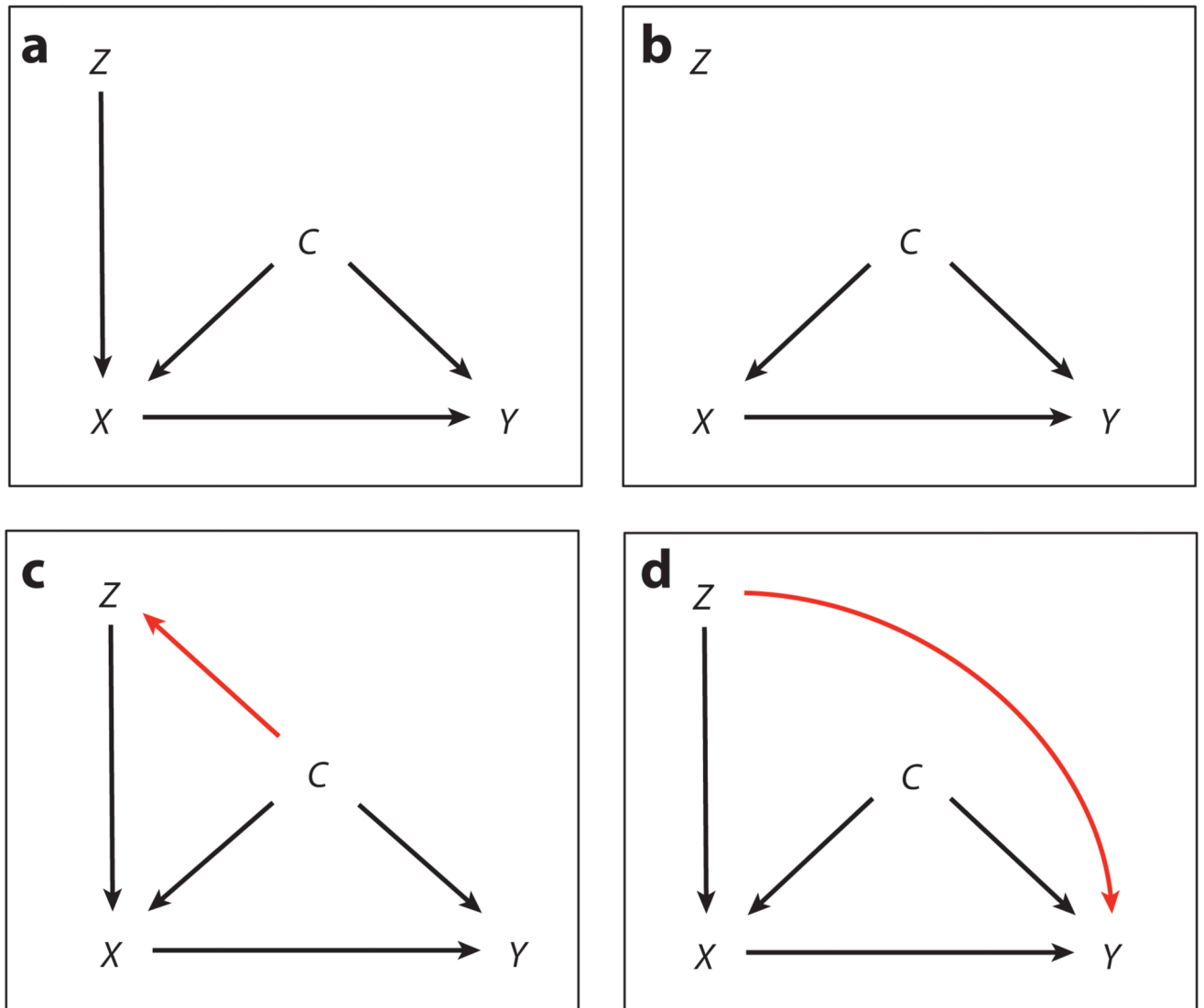
Figure 1. Directed acyclic graphs illustrating the assumptions of instrumental variable (IV) analysis.
