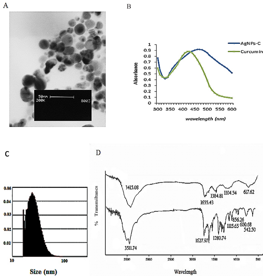
Figure 1. (A) TEM image of AgNPs-C, (B) Uv- visible spectrum from solution contains AgNO 3 and curcumin after passing 24 h, (C) particle size disruption of AgNPs-C, (D) comparing FTIR spectra from AgNPs-C (A) and pure curcumin (B) these spectra are very similar which indicated that curcumin coated the surface of silver nanoparticles.
