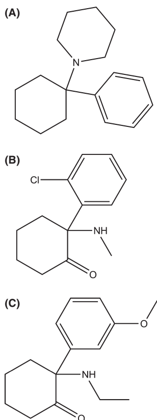
Figure 1 Chemical structures of (A) PCP, (B) KET, and (C) MXE.
