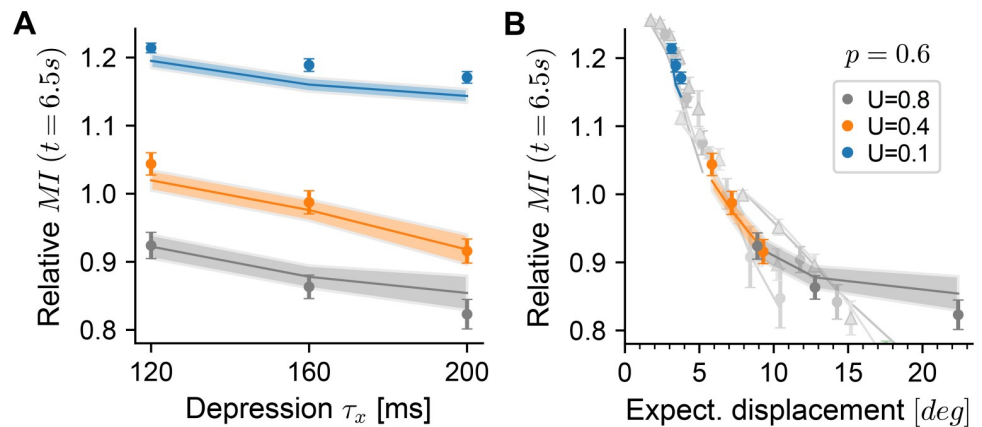
Fig 6. Short-term depression decreases memory retention. A Same as Fig 5B, for network simulations with varying \tau_x and U (see legend in panel B). MI is normalized to the same value as there. B Same as panel A, with x-axis showing the expected displacement. Gray data points and lines are the data plotted in Fig 5E. The facilitation time constant was kept constant at \tau_u = 650 ms.
