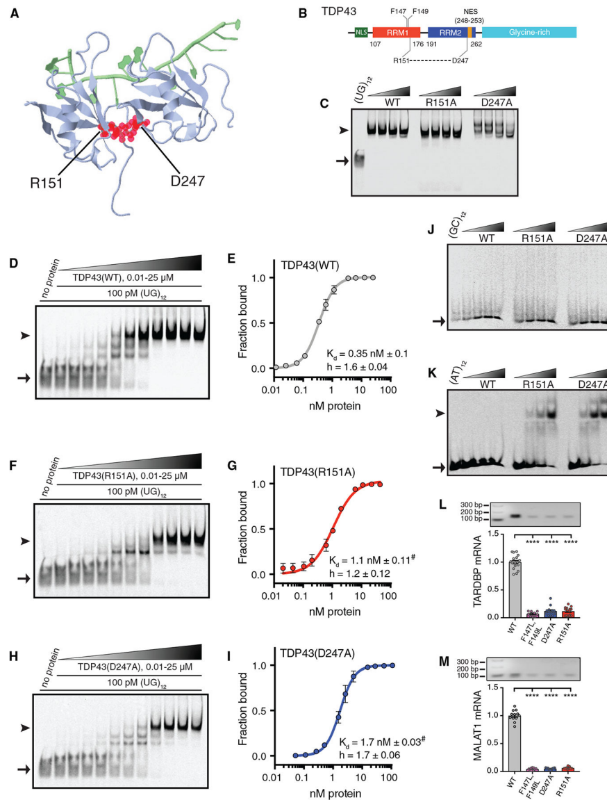
Figure 1. Disruption of the R151-D247 Salt Bridge Impairs Nucleic Acid Recognition by TDP43 (A) Structure of TDP43 RRM1 and RRM2, generated in FirstGlance in Jmol (PDB:4BS2), deposited by Lukavsky et al. (2013). TDP43 (blue) is shown in complex with UG-repeat RNA (green), highlighting the R151-D247 salt bridge (red). (B) TDP43 schematic depicting the RRM1-RRM2 salt bridge and F147-F149. (C) EMSA of increasing concentrations (12 fmol–4 pmol) of recombinant TDP43 variants mixed with labeled (UG)_{12} (100 pM). (D, F, and H) Increasing concentrations (0.01–25 \mu M) of TDP43(WT) (D), TDP43(R151A) (F), and TDP43(D247A) (H) were added to labeled (UG)_{12} (100 pM). (E, G, and I) K_d and h were calculated from 3 independent replicates for TDP43(WT) (E), TDP43(R151A) (G), and TDP43(D247A) (I). (J and K) EMSA of TDP43 variants at increasing protein concentrations (0.5–16 pmol) incubated with 100 pM of labeled (GC)_{12} (J) or (AT)_{12} (K).
