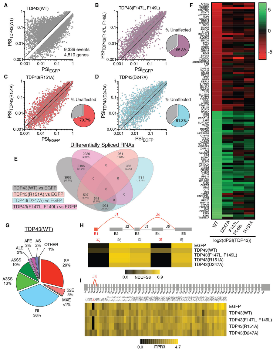
Figure 7. TDP43(WT) Overexpression Promotes Intron Retention and Exon Skipping
