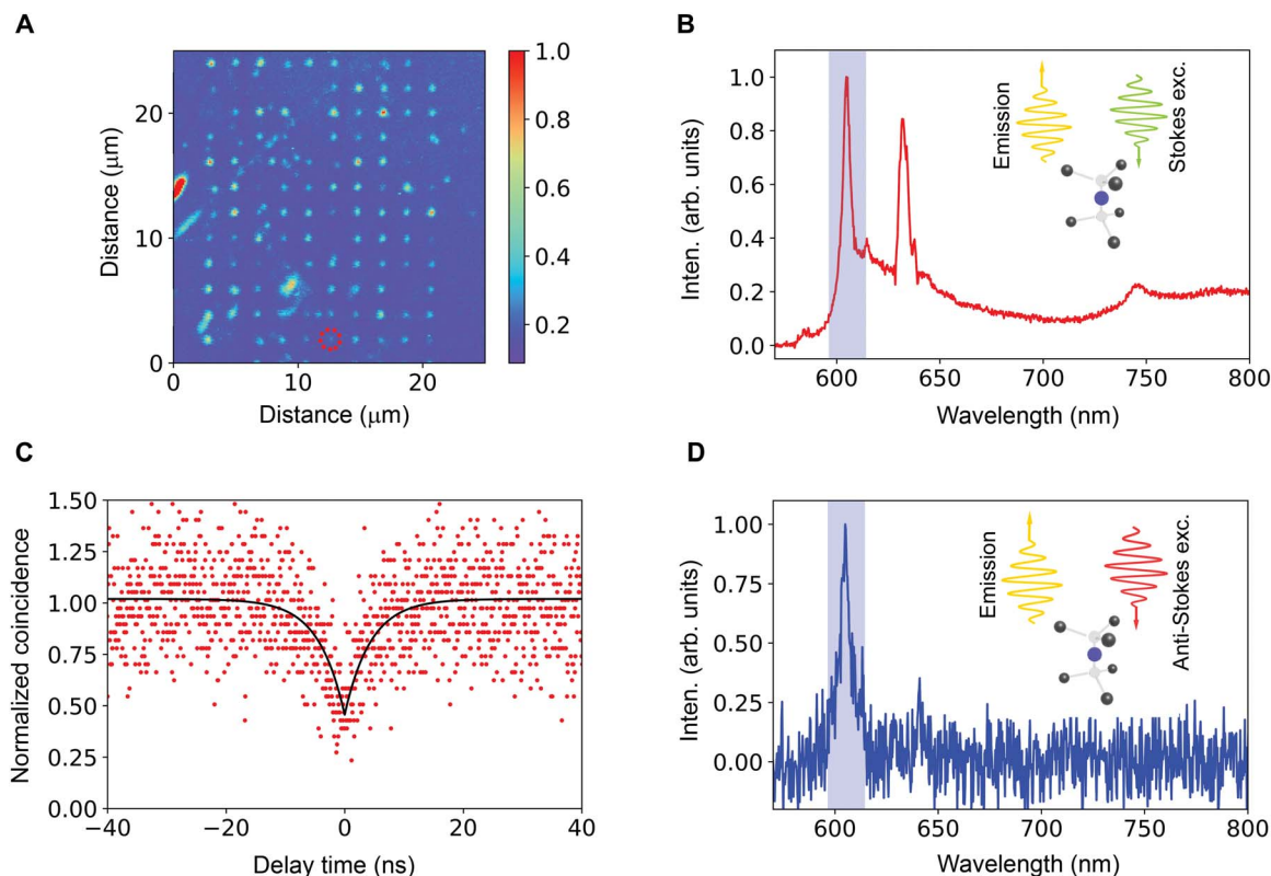
Fig. 2. Characterization of anti-Stokes emission from GeV color centers. (A) Confocal image of a 25\ \mu\text{m} \times 25\ \mu\text{m} bulk diamond sample showing emission from GeV color centers. Each spot has a different density of GeVs. The spot indicated by red circle is a single-photon GeV center as per analysis in (C). (B) PL spectrum acquired for the single center identified in (A). (C) Second-order autocorrelation function g^{(2)}(\tau) showing the sub-Poissonian statistic, at zero-delay time, indicative of a single photon source, g^{(2)}(0) < 0.5 [the value for g^{(2)}(0) is not background-corrected]. (D) Anti-Stokes PL spectrum acquired from the single GeV center in (A). The acquisition was carried out for 12 min, with laser excitation at 637 nm and 38 mW ( 23\ \text{MW}/\text{cm}^2 ) of power. A band-pass filter (represented as a semitransparent box around the ZPL of the spectrum) was used to acquire measurements in (C) and (D). The excitation wavelength used in (A) to (C) is 532 nm. The Stokes/anti-Stokes excitation wavelengths used in (D) are 532/637 nm.
