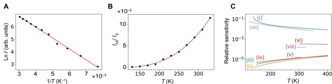
Fig. 3. Characterization of the anti-Stokes GeV-based nanothermometer. (A) Temperature dependence of the PL intensity signal upon anti-Stokes excitation (637-nm wavelength). The PL intensity was measured by monitoring the GeV's ZPL (605 nm) isolated with a band-pass filter. The data fit well the Arrhenius-type equation Ae^{-(E_a/k_B T)} , where the activation energy E_a = 102.96 meV is fixed to coincide with the difference in energy between the excitation laser and the GeV's ZPL. (B) Plot of the anti-Stokes to Stokes PL ratio as a function of temperature. The ratio fits an exponential curve: a + be^{-[c/(T-T_0)]} , granting the method an extremely high sensitivity. The error bars of plots in (A) and (B) are represented as vertical blue bars and are mostly equivalent to or smaller than the size of the data points. (C) Relative sensitivity plotted versus temperature for several different systems: our I_{AS}/I_S|_{GeV} measurement (i)*, the frequency shift of the GeV ZPL in our Stokes PL spectra (ii), the equivalent measurement from the literature (iii), the ZPL wavelength shift of the SnV (iv) and of the SiV center (v), the intensity of the NV ZPL (vi), the Raman I_{AS}/I_S ratio achieved for a bulk thermometer (vii), and the spectral shift of quantum dots (viii). The literature data are plotted over the entire temperature range demonstrated in each paper. The excitation wavelength used in (A) is 637 nm. The Stokes/anti-Stokes excitation wavelengths used in (B) are 532/637 nm.
