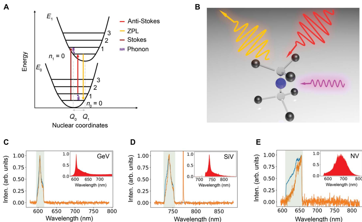
Fig. 1. Stokes and anti-Stokes luminescence processes for color centers in diamond. (A) Energy diagram of representative electronic and vibrational energy levels for a diamond color center. The arrows show the lower (higher) energy of the Stokes (anti-Stokes) photons with respect to the ZPL energy. In the anti-Stokes case, the additional energy is acquired via phonon(s) absorption. (B) Artistic representation of the anti-Stokes mechanism for a diamond color center, which absorbs a lower-energy photon (wavy line, red) and emits a higher-energy one (wavy line, orange) upon absorption of a phonon (wavy line, purple). (C to E) PL spectra of the ZPL for nanodiamond GeV (C), SiV (D), and NV (E) centers under Stokes (blue) and anti-Stokes (orange) excitation (the full PL spectrum under Stokes excitation is shown in the relative inset). The ZPLs (605 nm for GeV, 739 nm for SiV, and 639 nm for NV) are spectrally filtered by means of band-pass filters (semitransparent rectangular boxes). For each measurement in (C) to (E), the powers of the Stokes and anti-Stokes excitation lasers are the same; PL intensities are normalized to unity for display purposes: The measured values for anti-Stokes to Stokes PL intensity ratios for GeV, SiV, and NV centers are I_{AS}/I_S|_{GeV} = (8.4 \pm 3.3) \times 10^{-2} , I_{AS}/I_S|_{SiV} = (13.2 \pm 1.1) \times 10^{-2} , and I_{AS}/I_S|_{NV} = (11.9 \pm 2.8) \times 10^{-5} . The line at \sim 770 nm in (D) is the anti-Stokes excitation laser. The Stokes/anti-Stokes excitation wavelengths are 532/637 nm for (C), 637/770 nm for (D), and 532/720 nm for (E).
