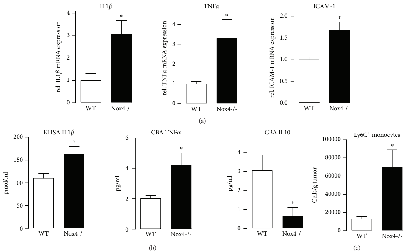
FIGURE 1: Nox4 deficiency favors inflammation in a murine tumor model. (a) Proinflammatory markers including the cytokines IL1 \beta and TNF \alpha and the adhesion molecule ICAM-1 were quantified by RT-qPCR in tumor tissue of WT and Nox4 -/- mice. (b) Proinflammatory markers IL1 \beta (ELISA) and TNF \alpha as well as IL10 (CBA: cytometric bead assay) as anti-inflammatory markers were measured in tumor tissue, n = 3 ; * p < 0.05 . (c) Single-cell suspension of tumor tissue was analyzed by FACS for Ly6C + monocytes; * p < 0.05 , n = 5-10 .
