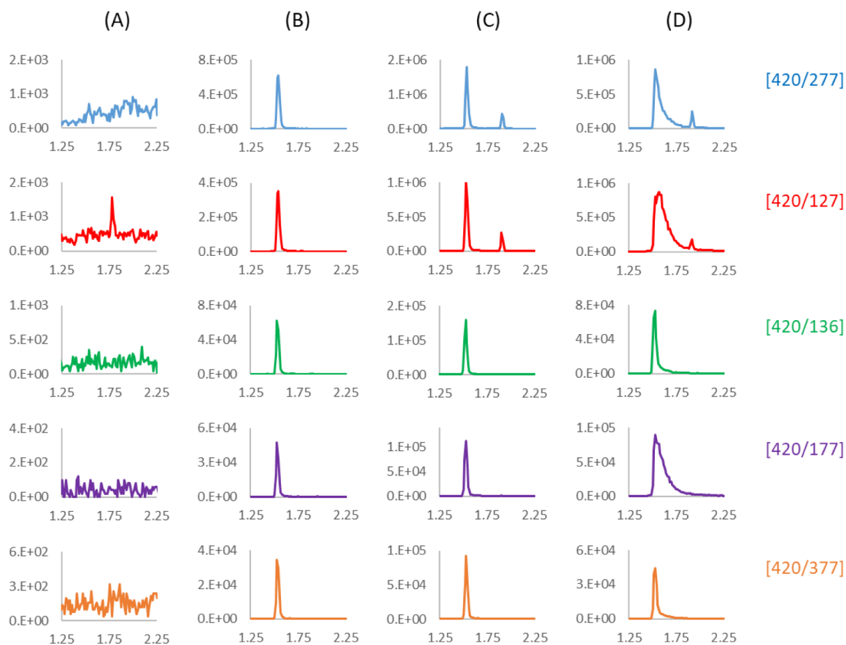
Fig. 3. Chromatograms from 5 MRM transitions [Q1/Q3] from a drug-free hair sample (Fig 3A) a drug-free hair sample spiked with DTG (Fig 3B) a clinical hair sample from subject on DTG regimen (Fig 3C) and a DTG solution in 50:50 methanol:water following exposure to sunlight for 3 hours (Fig 3D)
