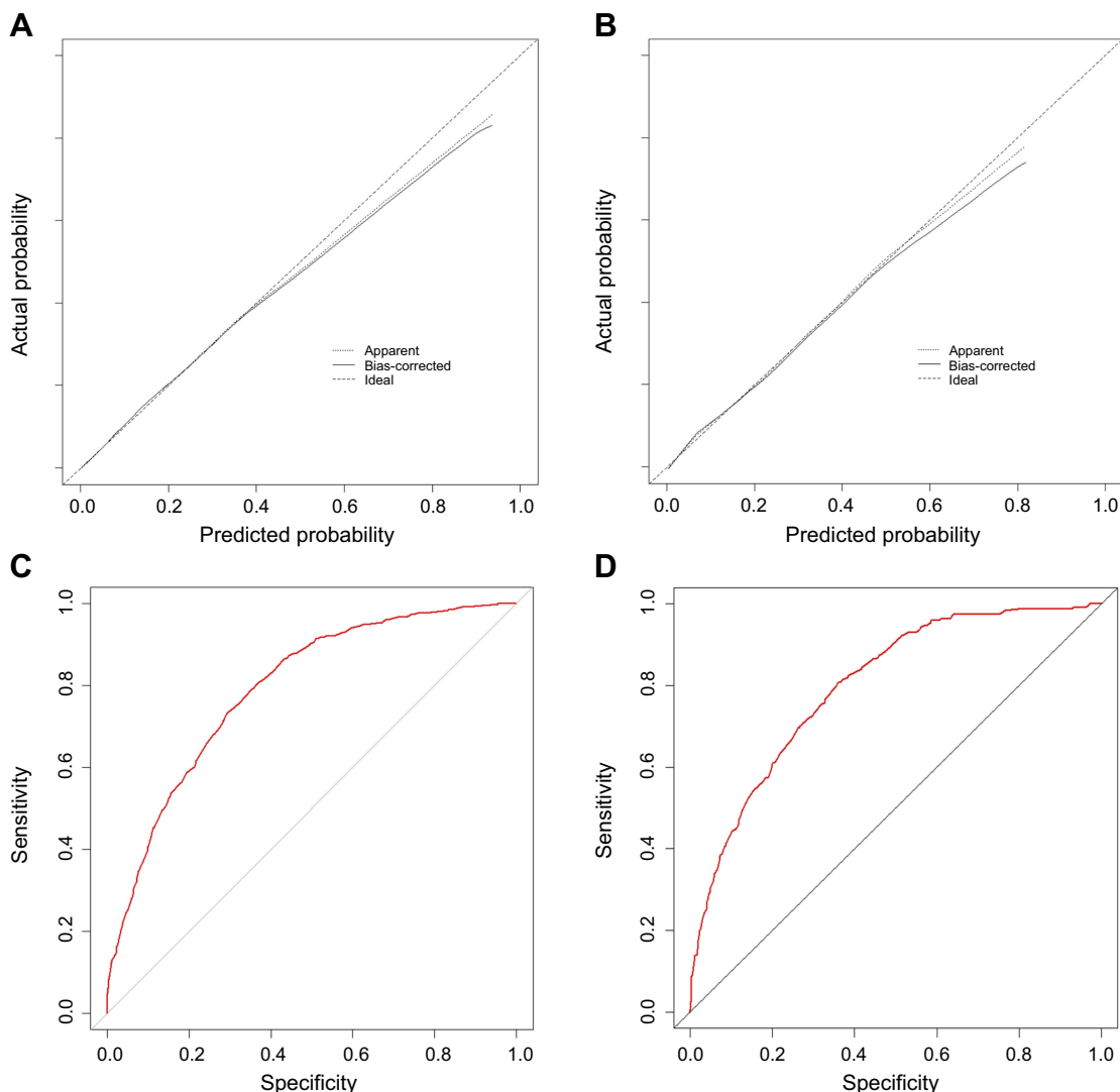
Figure 3 The calibration plots and ROC curves of model 2 in the training cohort (A and C, respectively) and validation cohort (B and D, respectively).
