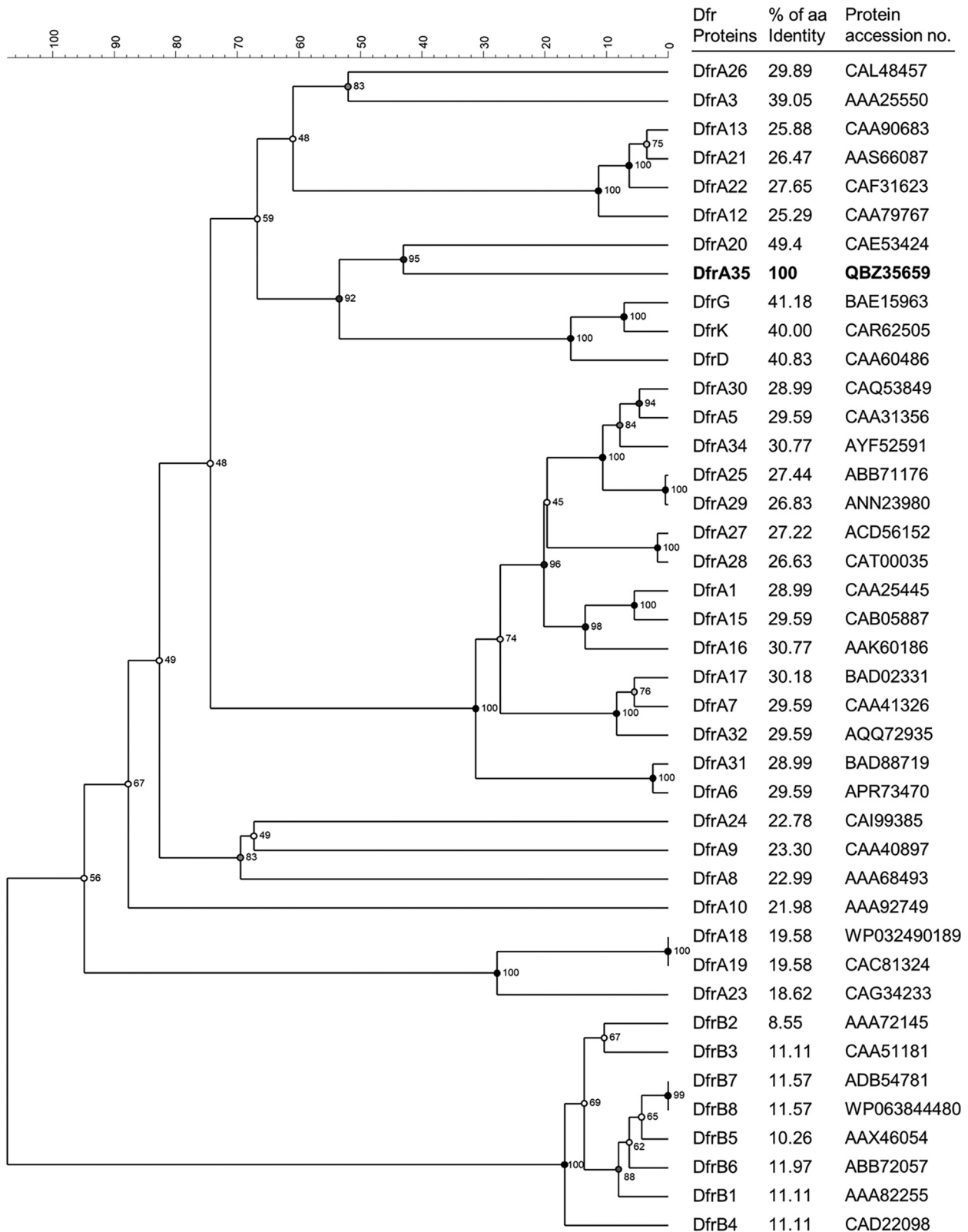
FIG 1 Phylogenetic tree of all known Dfr proteins, including the novel protein DfrA35. The tree was obtained by multiple alignment of amino acid sequences (without fast alignment) and the UPGMA clustering method with Jukes and Cantor correction using Bionumerics 7.6 (Applied Maths, Kortrijk, Belgium): multiple alignment with an open gap penalty (OG) of 100%, a unit gap penalty (UG) of 0%, a gap penalty of 100%, and 1,000 bootstrap values (nodes). Scala results are shown as distances. The percentages of amino acid sequence identity between DfrA35 and other Dfr proteins were determined by multiple sequence alignment with clustalW 2.1 (cost matrix Blosom) using Geneious prime 2019.1.1 (Biomatters, Ltd., Auckland, New Zealand).
