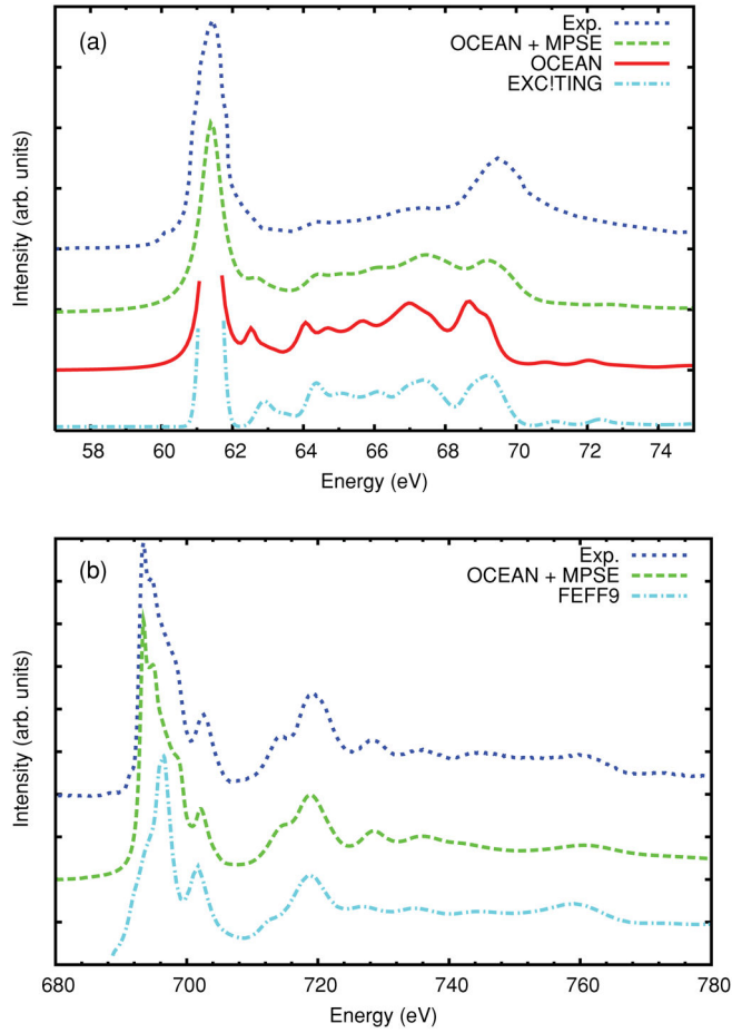
FIG. 2. (a) The x-ray absorption near-edge structure (XANES) spectra for the Li K edge of LiF (top) and (b) the F K edge (bottom). The BSE spectra (solid, red line) are compared to the same spectra convoluted with the MPSE correction (green, dashed line) and experiment 34,35 (Li data from Olovsson et al. 36 ) (blue, dotted line). In (a) the result of another BSE code, 36 (light blue, dashed-dotted line) and in (b) a calculation with the FEFF9 code (light blue, dashed-dotted line) are shown for comparison.
