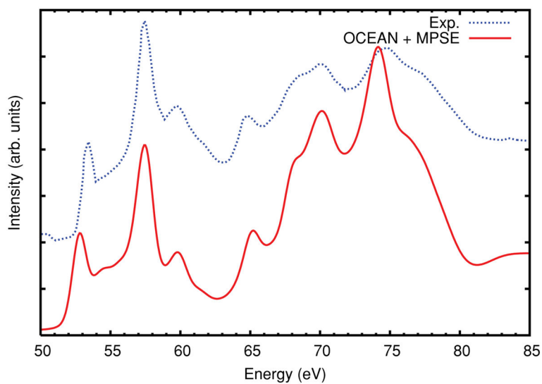
FIG. 5. Calculated XANES spectra for the Mg L_{2,3} edge of MgO compared with experimental reflection ( R^{1/2} ) data. 43 The calculated spectra has been broadened and by a Gaussian of 0.9 eV FWHM in addition to the MPSE.
