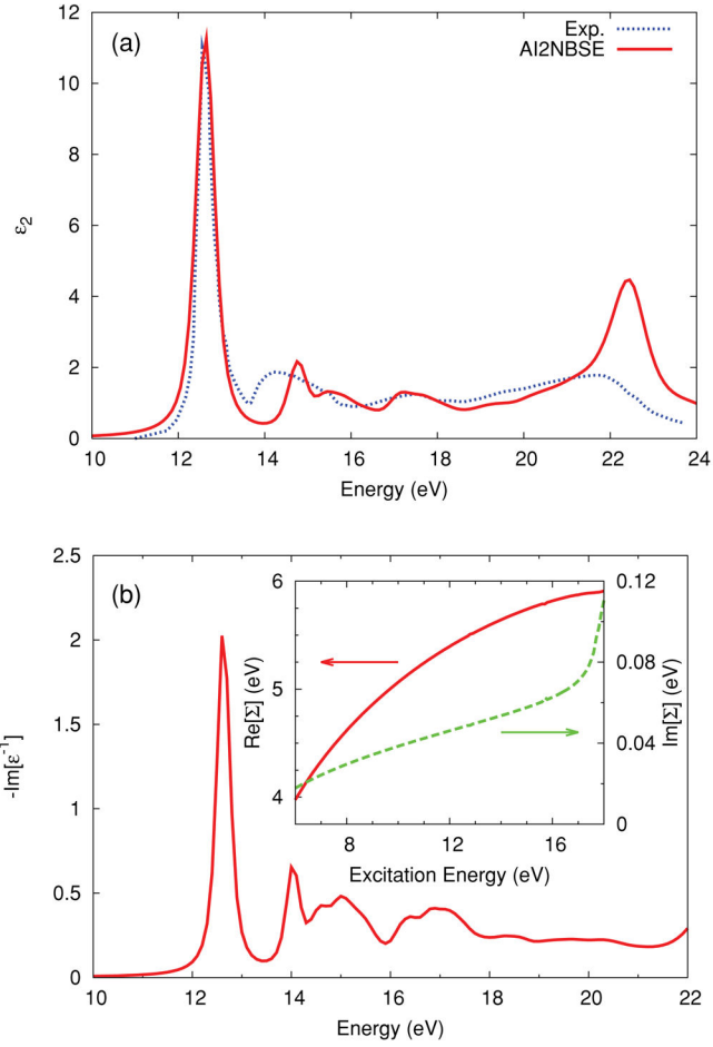
FIG. 1. (a) Imaginary part of the dielectric function (top) \epsilon_2(\omega) calculated with AI2NBSE (red, solid line) and experiment 30 (blue, dotted line) (data taken from Puschnig and Ambrosch-Draxl 31 ); and (b) loss function -\text{Im} \epsilon^{-1}(\omega) (bottom) with (inset) real and imaginary parts of the self-energy calculated from AI2NBSE. The self-energy is calculated from the loss function using the many-pole self-energy method (see text) and is shown relative to the valence band maximum. This self-energy is applied to the LiF K edges providing energy dependent broadening and energy shifts to correct the single-particle energies from DFT.
