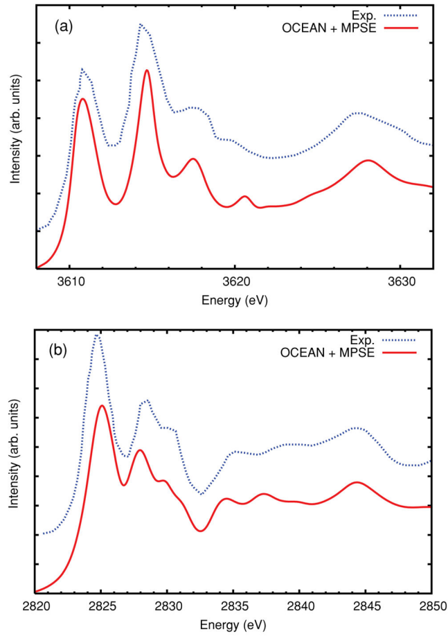
FIG. 4. (a) The K-edge XAS of potassium (top) and (b) the Cl K edge in KCl calculated with OCEAN (red, solid line) and compared to experimental results 42 (blue, dotted line).
