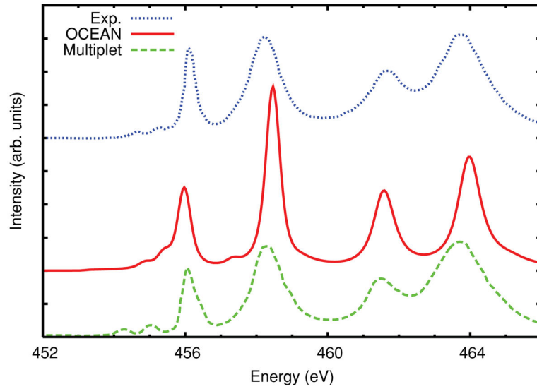
FIG. 6. Calculated XANES spectra for the Ti L_{2,3} edge of \text{SrTiO}_3 (red, solid line) compared to experimental data (blue, dotted line) and a multiplet calculation 44 (green, dashed line). Due to the close spacing of the edges the full MPSE was not included. Instead, the imaginary part of the self-energy was applied by aligning the onset with respect to each edge and including a core-hole lifetime (0.10 eV and 0.24 eV), shifting between the two at 461.5 eV. This lifetime broadening also neglects solid-state Coster-Kronig and phonon effects.
