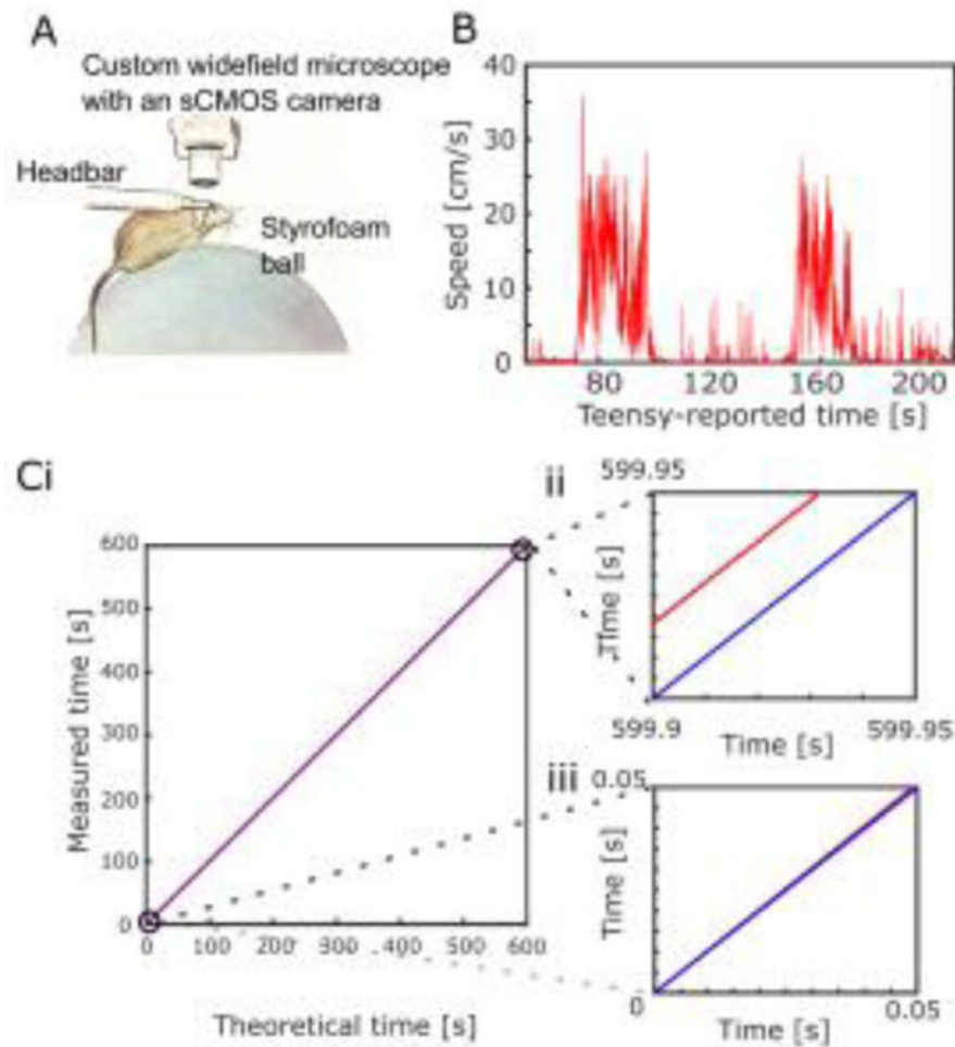
Figure 3. Temporal precision of the digital outputs in the motion tracking experiment. A. Illustration of the experimental setup, showing a mouse, awake and head-fixed, positioned on a Styrofoam ball. This can be positioned under an objective lens of a custom wide-field microscope equipped with a sCMOS camera. In this experiment, we did not perform calcium imaging with the sCMOS camera. (Illustration is modified from Gritton et al. (2019)). B. Example recording of a head-fixed mouse running on the spherical treadmill. C. Timing of digital pulses generated by the Teensy interface vs theoretical times of the digital pulses at exactly 20 Hz. Red line indicates linear model fit of experimental data, and blue line represents theoretic time with zero drift. The linear model of the experimental data estimates a slope of 1.000028937 + 0.000000002 ( t(11998) = 4.9e+08 , p < 0.001 , R^2 = 1 ; intercept = 0.0007593 + 0.00000007 , t(11998) = 1.1e+03 , p < 0.001 ). C(ii) and (iii) are zoomed in views of the beginning and end of the session.
