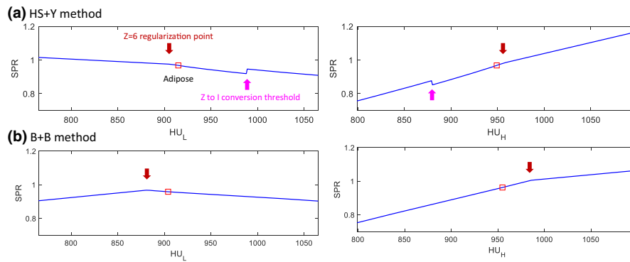
FIG. 4. Demonstration of the nonlinearities existing in the CT number to SPR map for (a) the HS + Y method and (b) the B + B method, respectively. Adipose tissue was selected here as an example. Red squares indicate the reference CT numbers of adipose. [Color figure can be viewed at wileyonlinelibrary.com]
