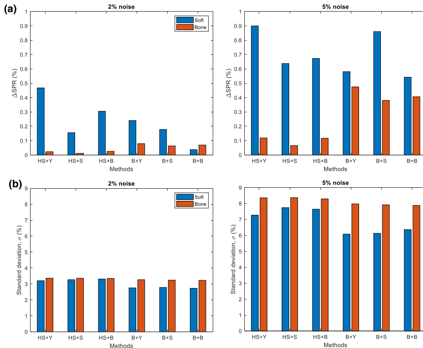
FIG. 10. Comparison of (a) SPR mean shift ( \Delta\text{SPR} ) and (b) variation ( \sigma_{\text{SPR}} ) of SPR when using different combinations of methods for the calculation of \rho_e and Z (Hunemohr-Saito (HS) and Bourque (B)) and the conversion of Z -to- I (Yang (Y), Saito (S) and Bourque (B)). Two different noise levels (2% and 5%) were applied to both \text{HU}_L and \text{HU}_H . CT numbers from 2000 individualized human tissue samples were used. [Color figure can be viewed at wileyonlinelibrary.com]
