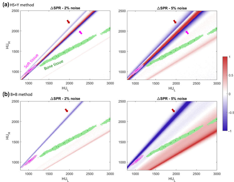
FIG. 6. Heatmap of the SPR mean shift ( \Delta SPR) using (a) the HS + Y method and (b) the B + B method at noise levels of 2% and 5%. Values are capped at (-1, 1) for ease of view as shown in the colorbar on the right. Grid size is 10 \times 10 . Magenta dots mark soft tissues and green dots mark bone tissues from the ICRU 44 reference. Shaded areas of each color denote 2000 individualized human tissue population. Arrows indicate the regions with hard threshold as shown in Fig. 4. [Color figure can be viewed at wileyonlinelibrary.com]
