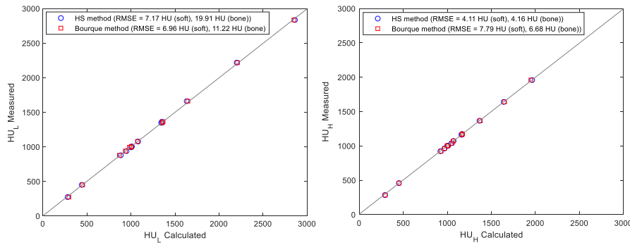
FIG. 2. Calculated vs measured CT numbers of the Gammex phantom inserts using the HS method (circle) and the Bourque method (square) for HU_L (left) and HU_H (right). A 45° line (gray) is drawn as a reference. [Color figure can be viewed at wileyonlinelibrary.com]
