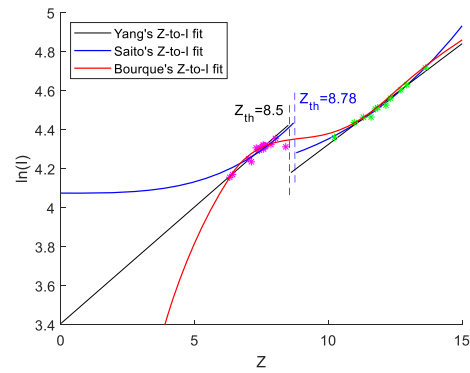
FIG. 1. Z -to- I conversions proposed by Yang (Y), Saito (S), and Bourque (B). All three methods were fitted using the ICRU 44 reference human tissues. Magenta asterisks indicate soft tissues and green asterisks indicate bone tissues. [Color figure can be viewed at wileyonlinelibrary.com]
