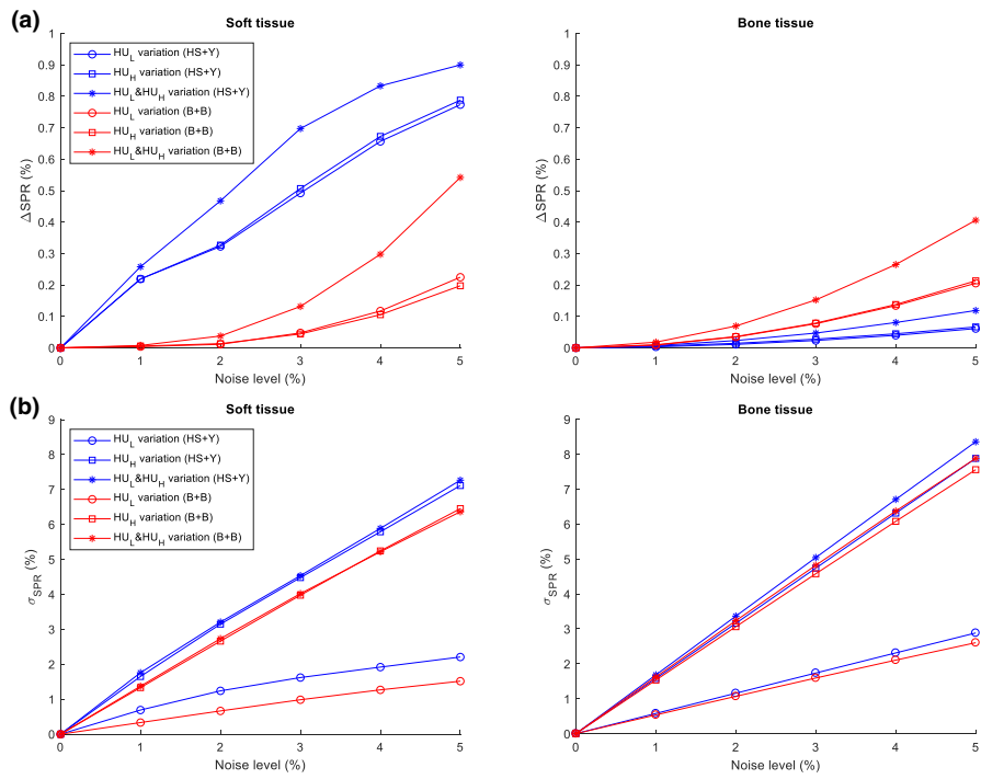
FIG. 8. Impact of noise on the SPR estimation manifested as (a) the shift of mean SPR ( \Delta_{SPR} ) and (b) the variation ( \sigma_{SPR} ) of SPR with varying levels of noise on HU_L , HU_H , or both. CT numbers from 2000 individualized human tissue samples were used. [Color figure can be viewed at wileyonlinelibrary.com]
