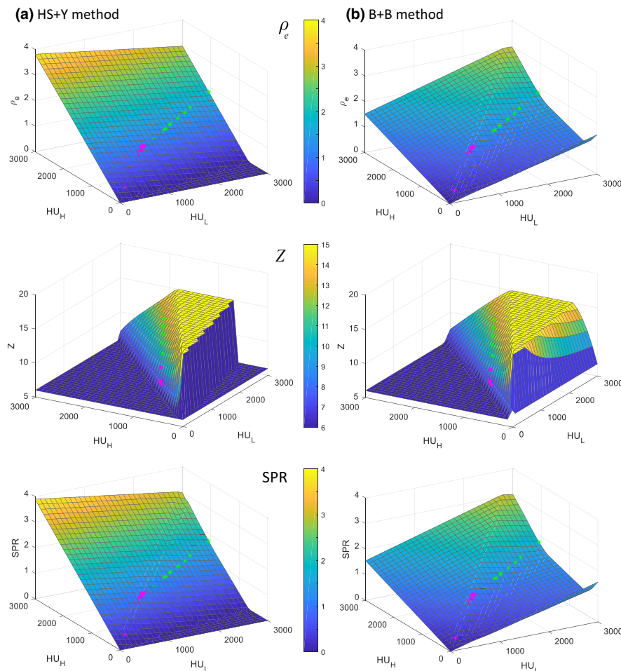
FIG. 3. \rho_e , Z , and SPR of (a) the HS + Y method and (b) the B + B method with all the possible combinations of CT numbers within (0, 3000) with grid size of 100. Magenta and green asterisks represent soft tissues and bone tissues, respectively, selected from ICRU 44 (Table II). Note that all negative or complex values were forced to zero and Z was regularized to (6, 15) to avoid unrealistic values. [Color figure can be viewed at wileyonlinelibrary.com ]
