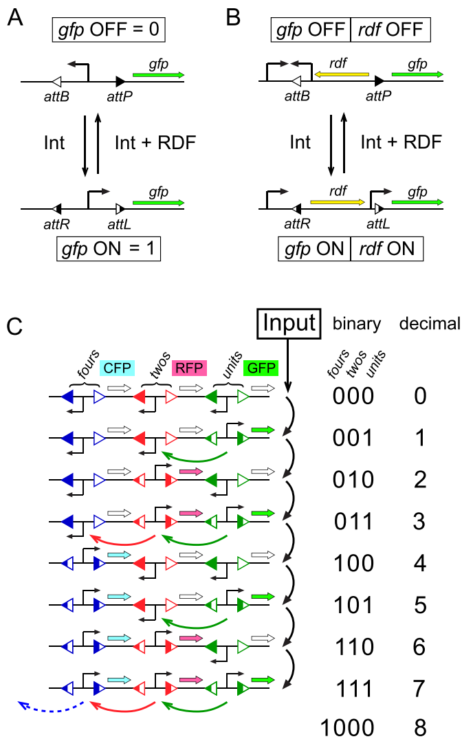
Figure 1. Inversion switches for binary memory and counters. (A) The integrase (Int) protein on its own catalyzes recombination between DNA sites attP and attB to create two new sites, attL and attR . Recombination between attL and attR only occurs if the recombination directionality factor (RDF) and integrase are both present. If att sites are in inverted repeat on either side of a promoter, recombination will reverse the orientation of the promoter and control transcription of a gene outside the invertible DNA segment (e.g. the gene for green fluorescent protein (GFP)). The two states of the inversion switch can be thought of as representing the binary digits 0 and 1. (B) Expression of the RDF can be placed under the control of the switch so that it is expressed in the LR state but not the PB state. A pulse of integrase expression should toggle the state of the switch from PB→LR or LR→PB. (C) Three inversion switches based on orthogonal integrases can be used to represent any binary number from 0 to 111 (0 to 7 decimal). The state of each switch is output through expression of three different fluorescent proteins, exemplified here as green-, red- and cyan fluorescent proteins (GFP, RFP and CFP). The figure shows the design for a binary ‘ripple’ counter that will step sequentially through all binary numbers between 000 and 111 in response to a repeated input signal. Each input signal (black arrows) toggles the state of the ‘units’ (GFP) switch so that it alternates between PB (0) and LR (1) states. As the units switch changes from 1 to 0, it sends a signal (green arrows) to toggle the ‘twos’ (RFP) switch, which in turn sends a signal (red arrows) to toggle the ‘fours’ (CFP) switch as it changes from 1 to 0.
